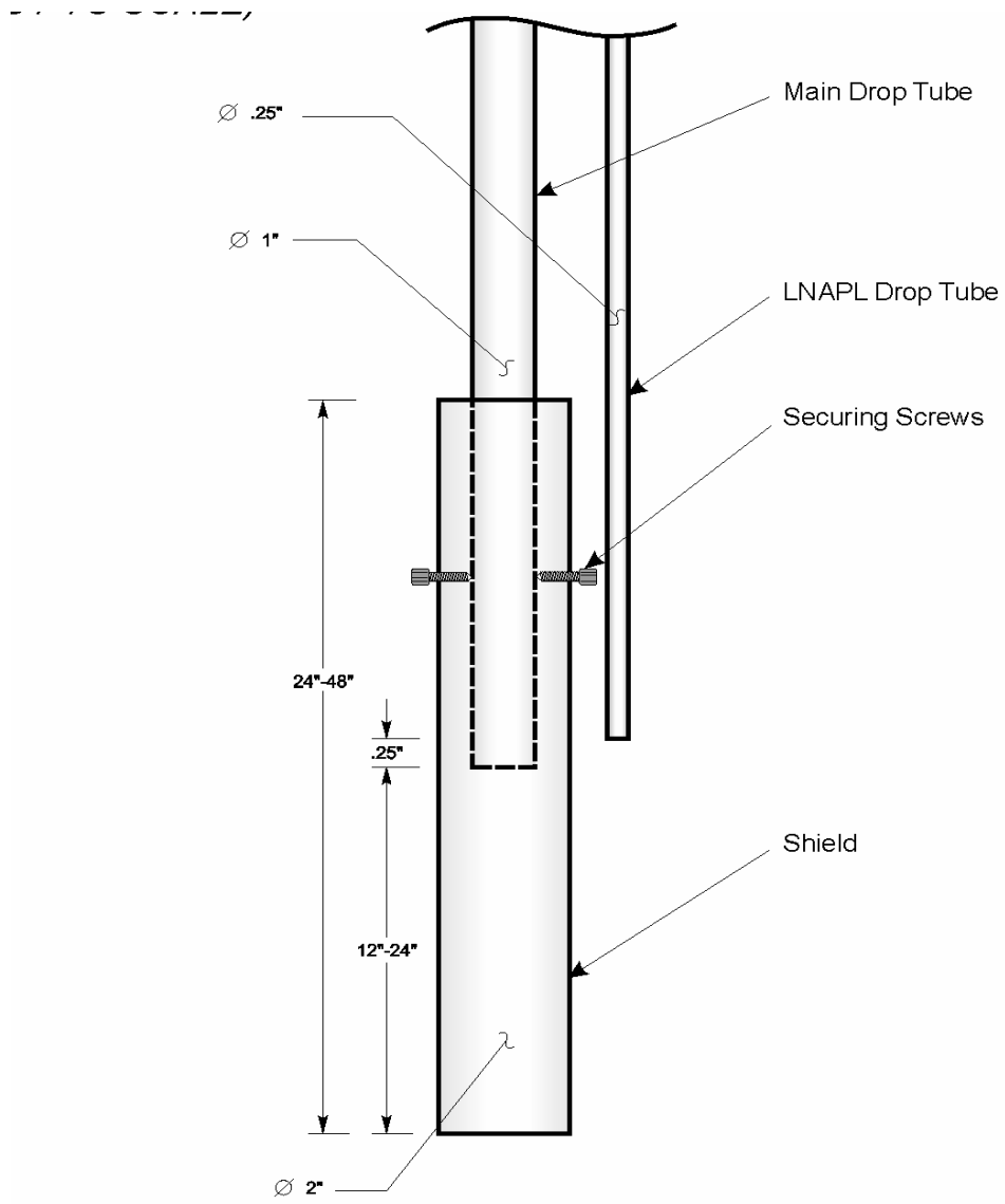
Figure 5. Engineering Design of the Dual Drop Tube System
