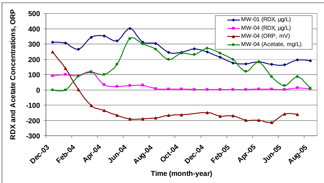
Figure 30. Comparison of RDX and acetate concentrations and ORP levels. Well MW-01 was the upgradient well and Well MW-04 was within the treatment zone.
