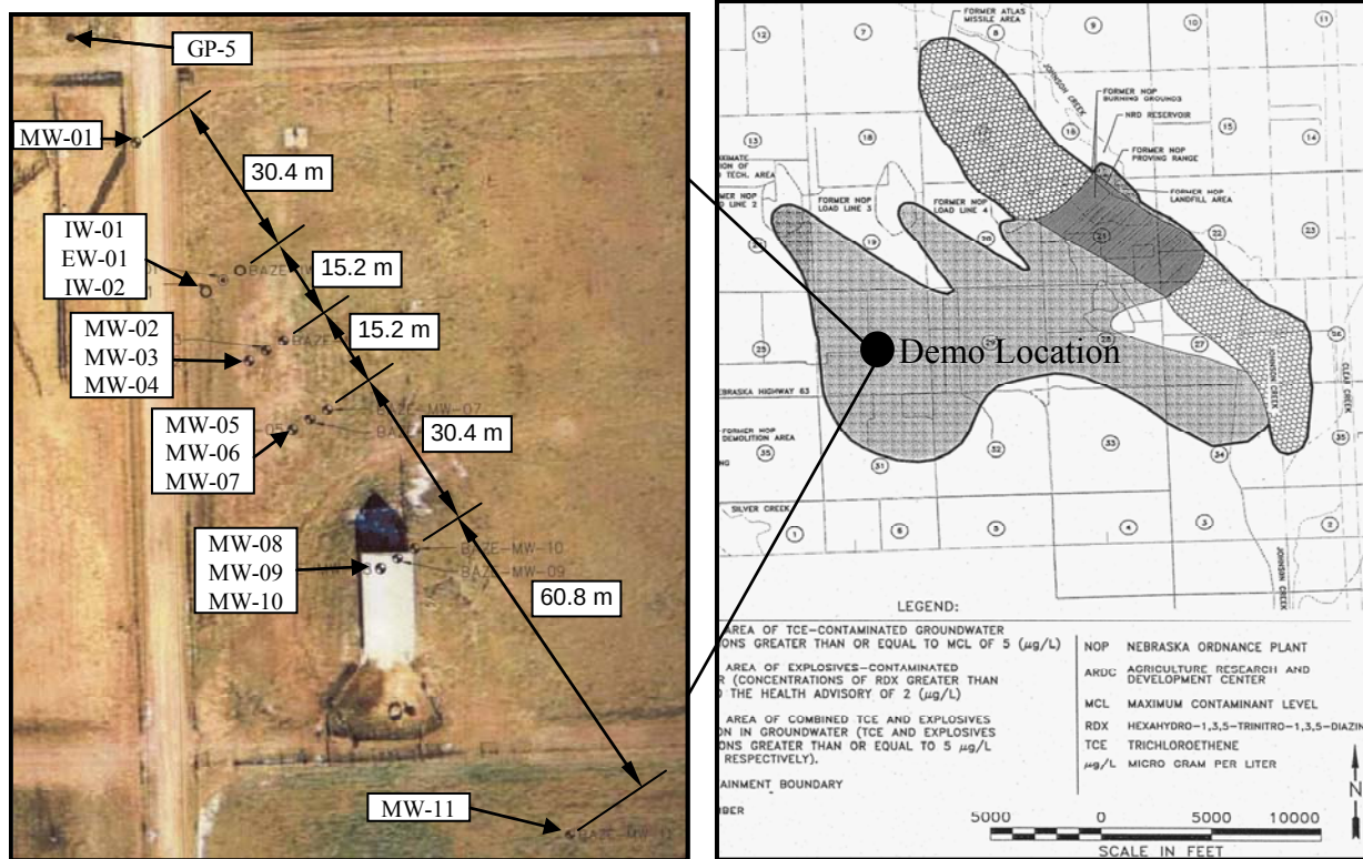
Figure 11. Extent of groundwater contamination (Woodward-Clyde 2000) and BAZE well and demonstration locations.
