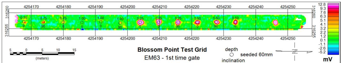
Figure 3-8 False color images showing EM63 data (1st time gate) over lane Z of the Blossom Point test grid. The symbols identify seeded 60mm mortars.
