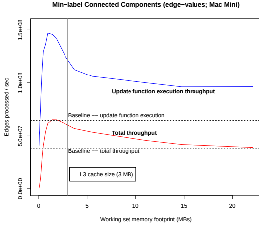
(c) Mac Mini: Connected Components / edge values
