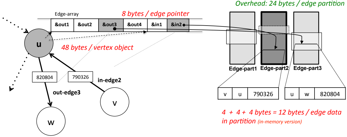
Figure A.2: Memory footprint of the Parallel Sliding Window’s in-memory version for vertex-centric computation. Each vertex object requires 48 bytes of memory: (1) pointers to beginning of in- and out-edge arrays (2) number of in- and out-edges; (3) pointer to vertex’s value (not shown); (4) vertex ID; (5) C++ object overhead. Each edge currently loaded into memory is referenced from the edge-array. In this example, each edge stores a integer ID of 4 byte and IDs, in addition to the the source and destination vertices. Two edges of the vertex (in-edge2 and out-edge3) are shown in detail. Each edge partition has an additional 24 byte overhead. Note: the internal edge partition structure is different for GraphChi and GraphChi-DB.
