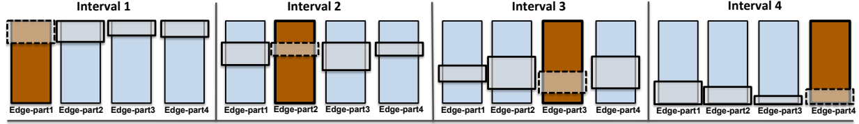
Figure 3.2: A visualization of the stages of one iteration of the Parallel Sliding Windows method. In this example, vertices are divided into four intervals, each associated with an edge partition. The computation proceeds by constructing a subgraph of vertices one interval at a time. The in-edges for the vertices are read from the memory-partition (in dark color) while out-edges are read from each of the sliding partitions . The current sliding window is pictured on top of each partition.
