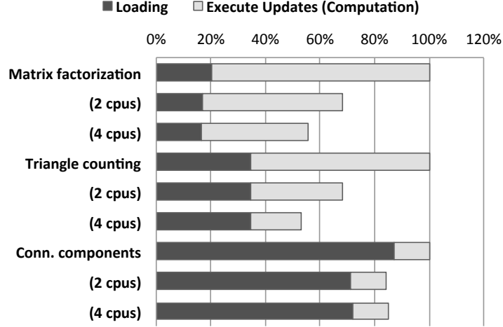
Figure 3.6: Relative runtime when varying the number of threads used by GraphChi. The experiment was done on a MacBook Pro (mid-2012) with four cores.
