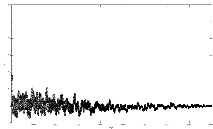
Figure 8.2: The Autocorrelation Plot
