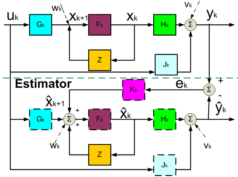
Figure 6.1: The Kalman Filter Flow Chart
