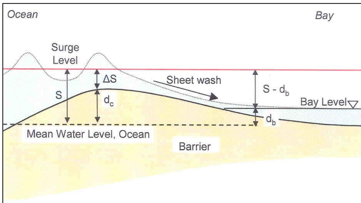
Figure 7. Definition sketch showing cross section of a barrier beach subject to overwash by overflow where barrier is fully inundated.
