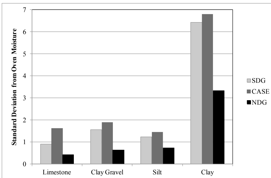
Figure 34. Standard deviation of oven-dried moisture from calibrated moisture content.
