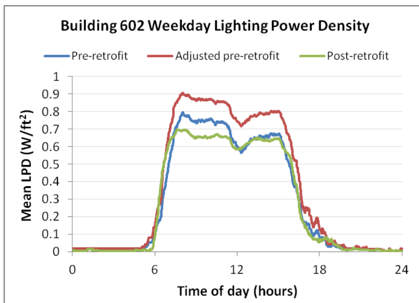
Figure 7. Building 602 mean weekday LPD for pre-retrofit, adjusted pre-retrofit, and post-retrofit.
