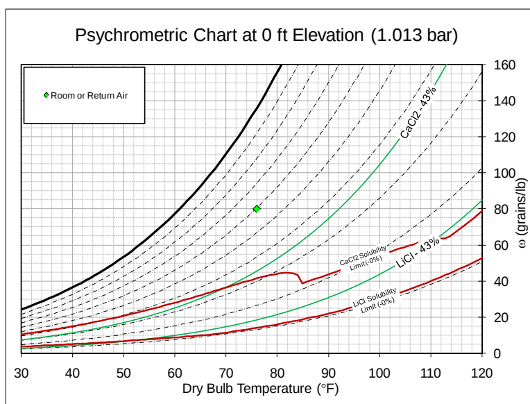
Figure 1. Psychrometric chart showing the dehumidification process using desiccants.
