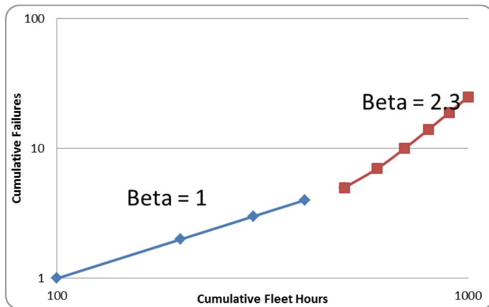
Figure 4.4. Example of Crow-ASMAA Plot
