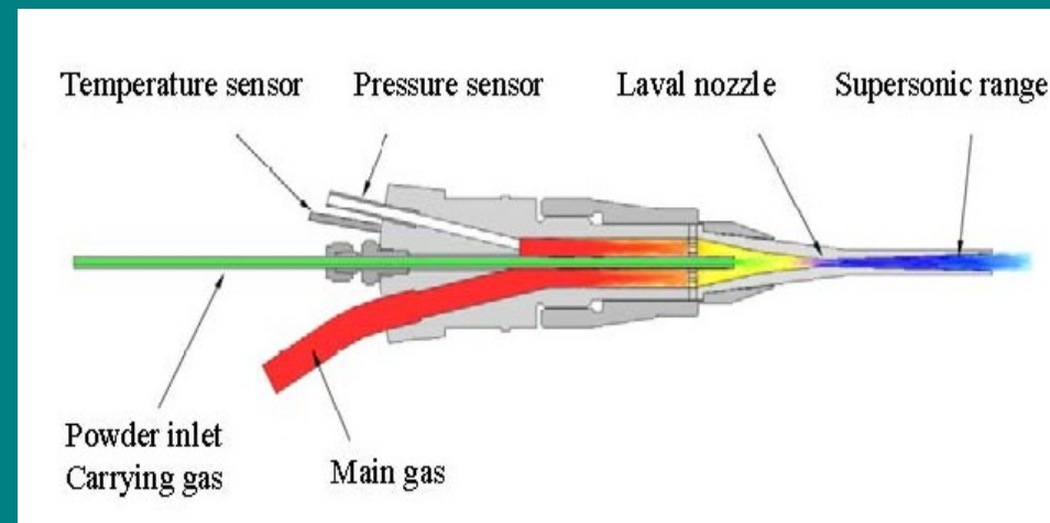
Schematic of the SPD gun and nozzle
