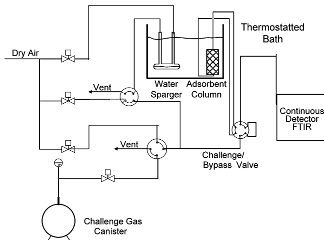
Figure 1. Microbreakthrough system schematic.
