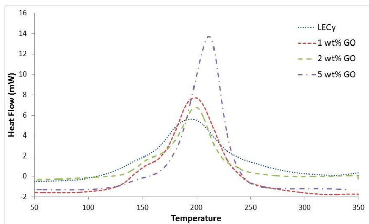
Figure 5. Dynamic Differential Scanning Calorimetry (DSC) of LECy monomer and LECy monomer-graphene oxide mixtures.
