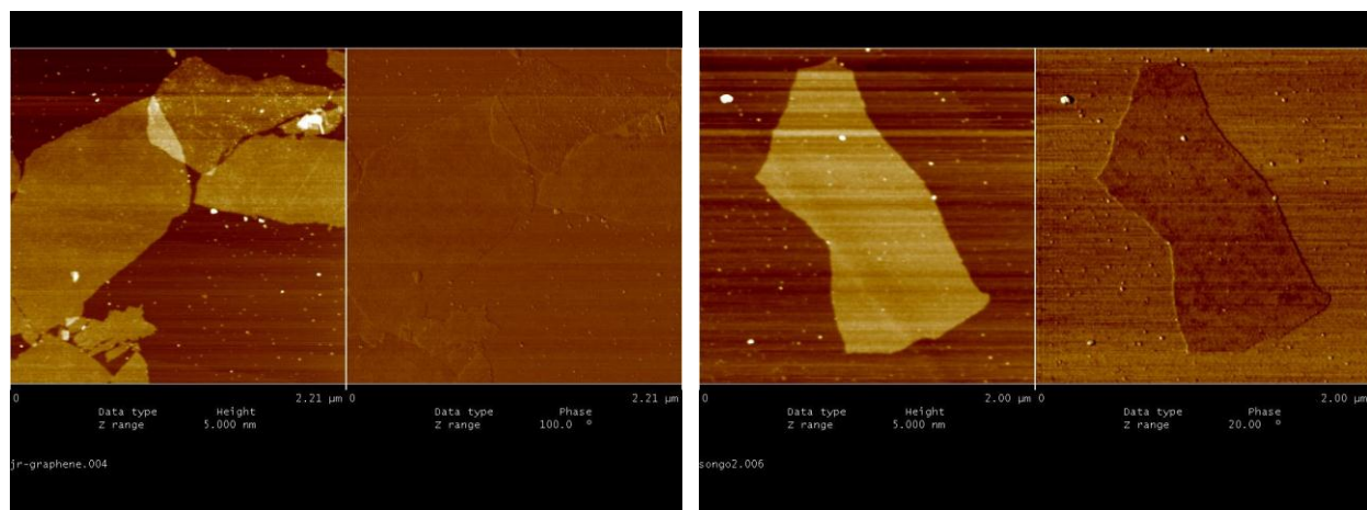
Figure 2. AFM images of graphene oxide on freshly cleaved silica. Images are 2 \mu\text{m} x 2 \mu\text{m} .
