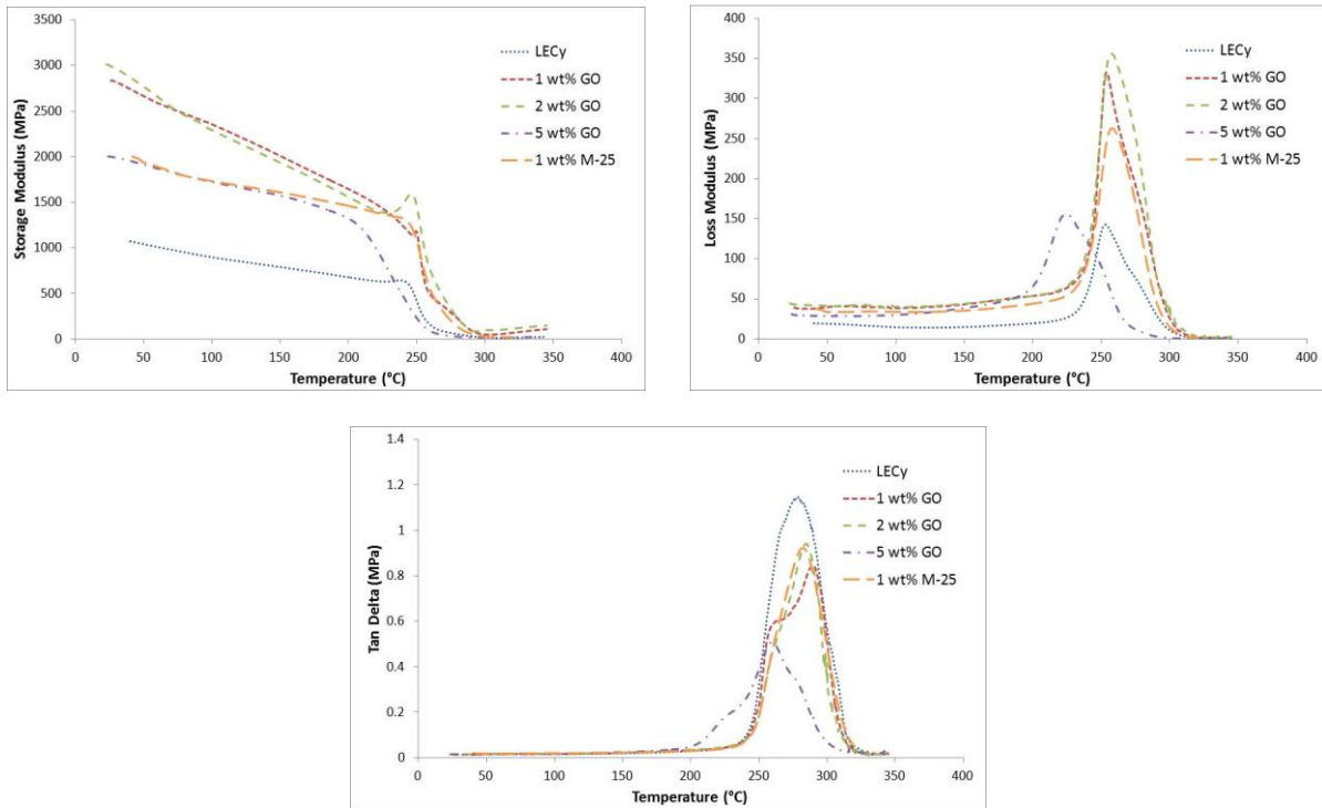
Figure 8. DMA graphs (first heating cycle) of LECy-GO and LECy-graphite composites.
