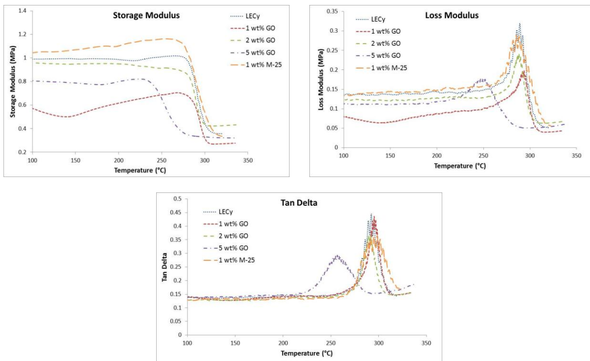
Figure 7. TMA graphs (second heating cycle) of LECy-GO and LECy-graphite composites.
