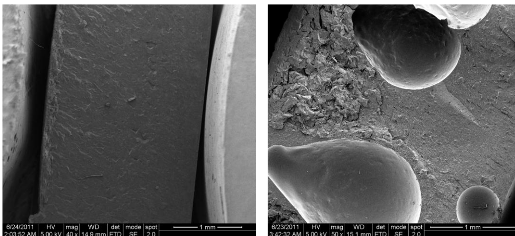
Figure 12. Low magnification SEM micrographs of the fractured surface of 1 wt% (left) and 5 wt% (right) GO LECy composites.
