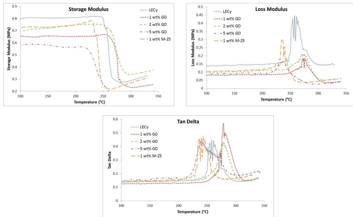
Figure 6. TMA graphs (first heating cycle) of LECy-GO and LECy-graphite composites.
