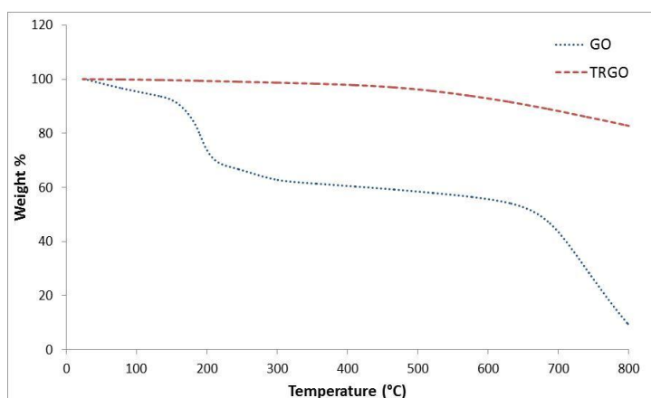
Figure 4. TGA of graphene oxide (GO) and thermally reduced graphene oxide (TRGO) in nitrogen.
