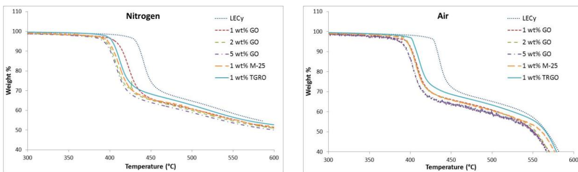
Figure 10. Weight loss vs. temperature for GO, M-25 graphite and TRGO composites in Nitrogen (left) and Air (right) atmosphere.
