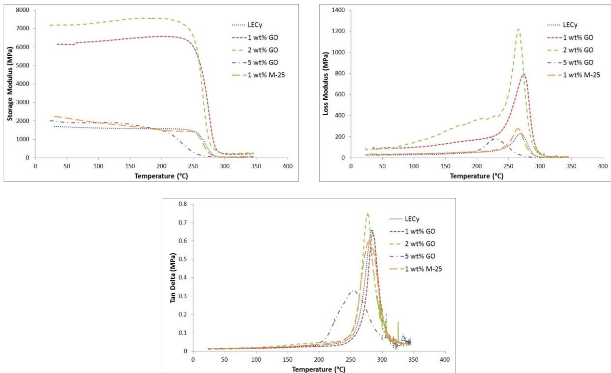
Figure 9. DMA graphs (second heating cycle) of LECy-GO and LECy-graphite composites.
