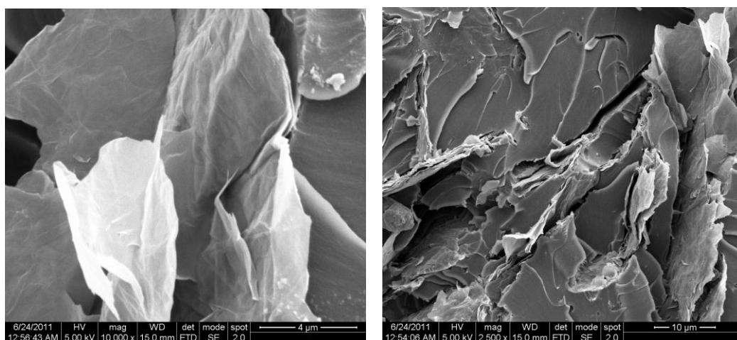
Figure 11. SEM micrographs of the fractured surface of 2 wt% GO LECy composite.
