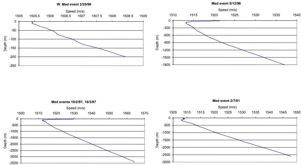
a. Climatological profiles from GDEMV 3.0
