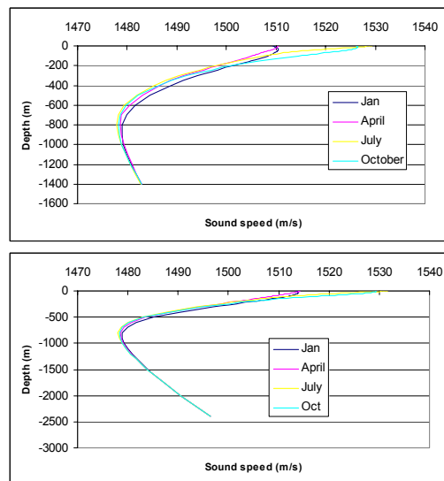
a. Climatological profiles from GDEMV 3.0
