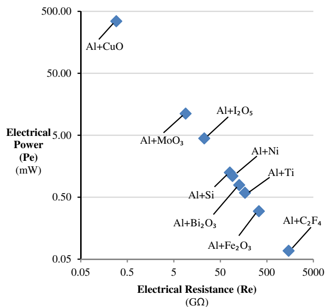
Fig. 5. Variation of electrical power with electrical resistance.
