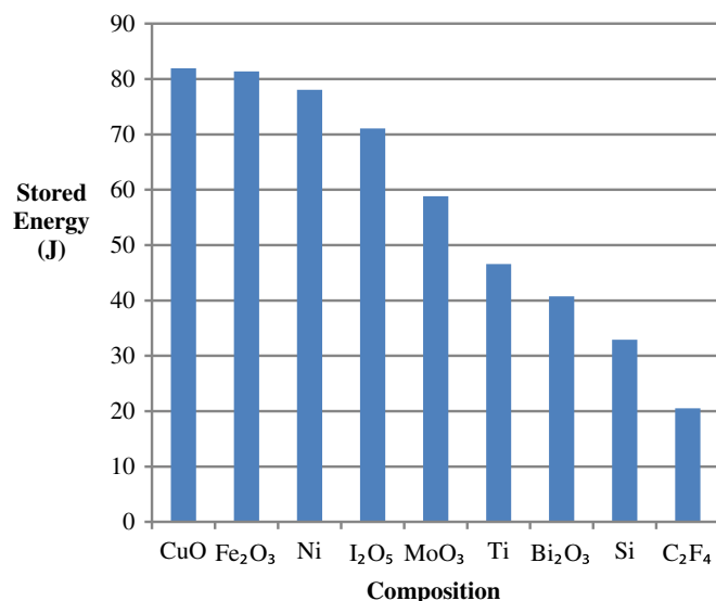
Fig. 6. Thermal energy stored for each oxide.
