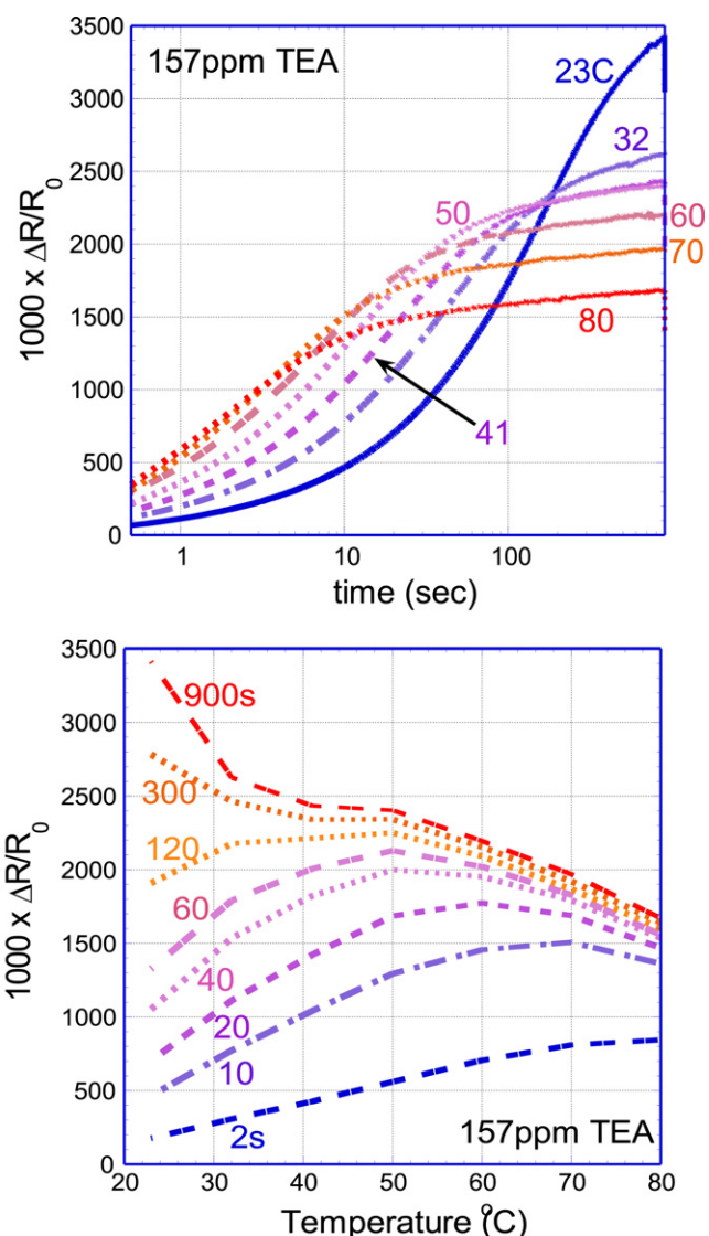
Fig. 8. (a.) Transient responses of an MHA-MIME sensor to a single 15 min dose of TEA (at 157 ppm) with temperature as a parameter. (b.) Cross-plot of the data in (a) with the time elapsed from the start of the exposure used as a parameter.
