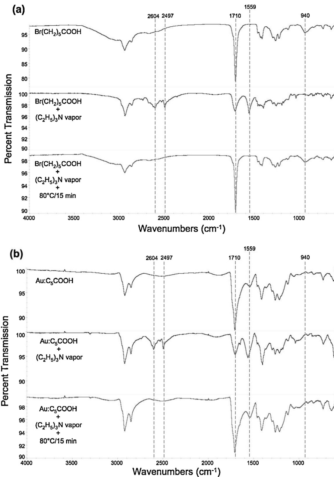
Fig. 3. IR absorption spectra (in percent transmission) of (a) a Br(CH 2 ) 5 COOH film and (b) an Au:C 5 COOH cluster film before, after exposure to TEA, and following heat treatment.
