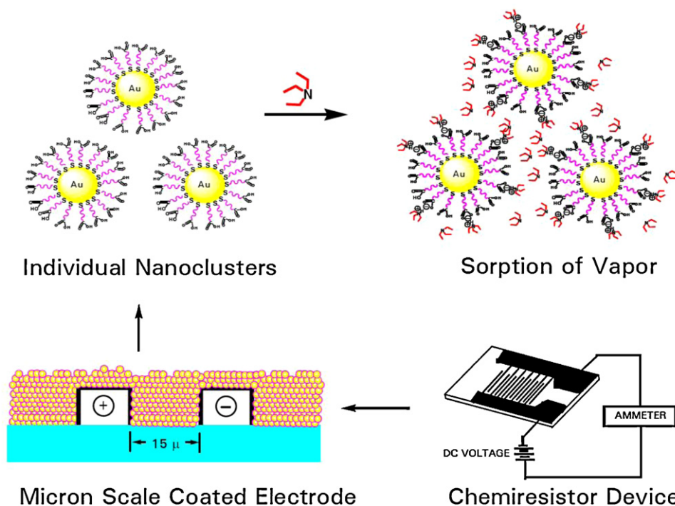
Fig. 1. Depictions of the COOH-functionalized nanoclusters and their integration into a MIM sensor.
