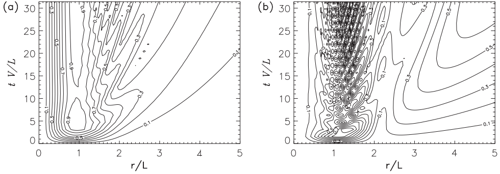
Figure 14. Hovmöller plots of \max_{\lambda}[q^{ab}](r, t) under sustained external strain. The fields are normalized by their maximum value near r=L and t=3L/V : (a) CYCLONE (max value = 0.736 fV/L ) and (b) ANTICYCLONE (max value = 0.095 fV/L ). The contour interval is 0.1.
