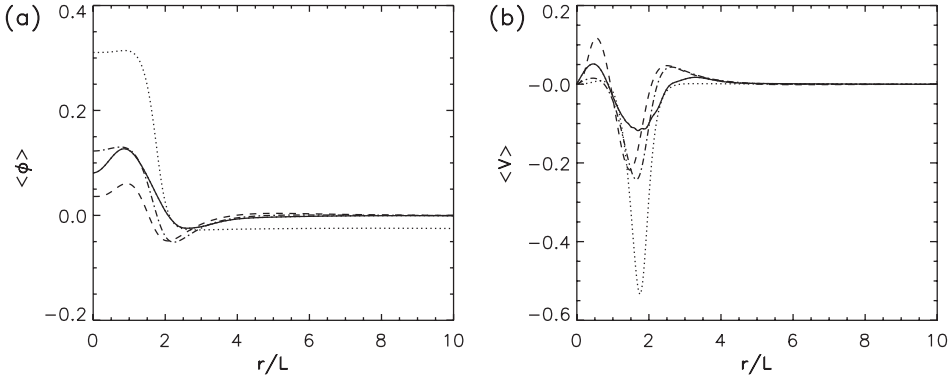
Figure 10. Net vortex change in (a) \langle\phi\rangle(r) normalized by m^2 V f L and (b) \langle v\rangle(r) normalized by m^2 V over the full time integration, including both the impulsive straining and relaxation phases. CYCLONE = solid line; ANTICYCLONE (with the sign reversed) = long-dash line; QG = dash-dot line; BT = dot line.
