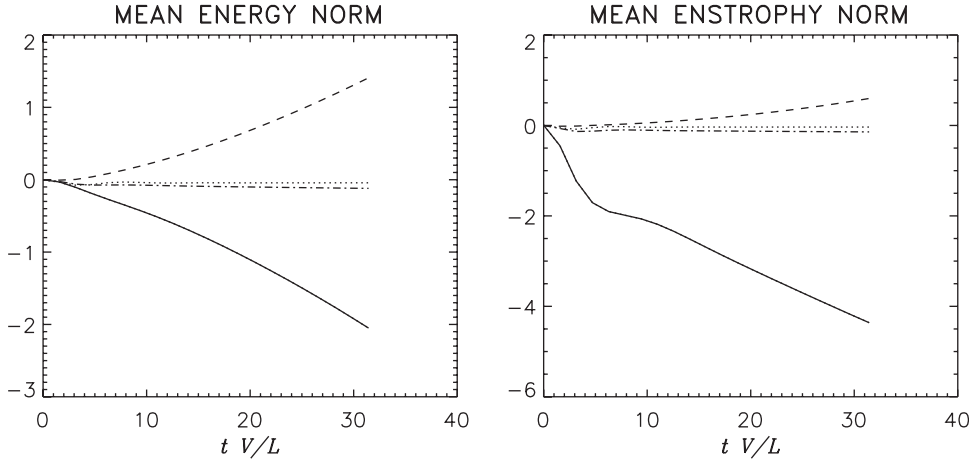
Figure 12. History of the vortex change norms for (left) energy, \Delta \bar{E}_{swe}(t) , and (right) potential enstrophy, \Delta \bar{V}_{swe}(t) , for the primary cases with sustained external strain: CYCLONE = solid line; ANTICYCLONE = long-dash line; QG = dash-dot line; and BT = dotted line. Normalizations are in table 1.
