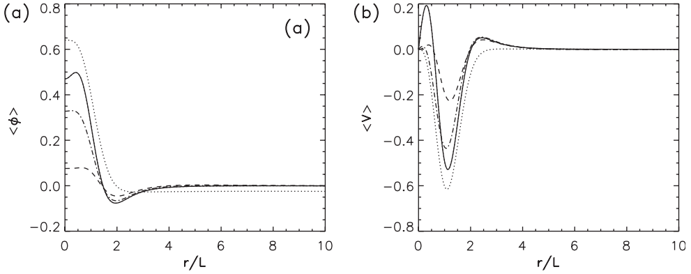
Figure 5. (a) \langle \hat{\phi} \rangle_M(r) normalized by VfL and (b) \langle \bar{v} \rangle_M(r) normalized by V for the standard cases defined in section 3: CYCLONE = solid line; ANTICYCLONE (with the sign reversed) = long-dash line; QG = dash-dot line; BT = dot line. The radius is normalized by L .
