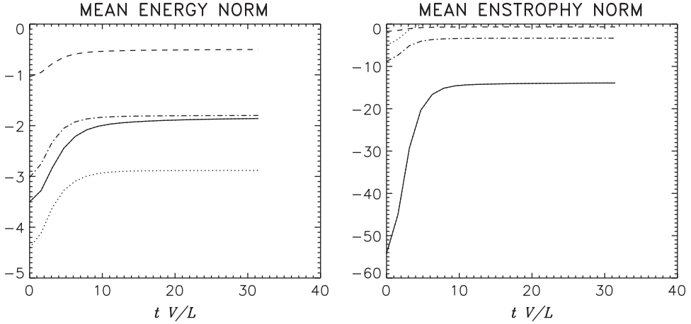
Figure 2. History of the normalized vortex change norms for (left) energy, \Delta \bar{E}_{\text{swe}}(t) , and (right) potential enstrophy, \Delta \bar{V}_{\text{swe}}(t) , for the primary cases with impulsive strain: CYCLONE = solid line; ANTICYCLONE = long-dash line; QG = dash-dot line; and BT = dotted line. Normalizations are in table 1. All curves start at zero for t=0 , but the strain-weakening period is so brief (i.e., t_{\text{max}} V/L = 0.014 ) on the scale of the plot that they appear to start at their post-strain, minimum values.
