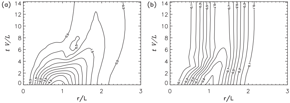
Figure 7. Hovmöller plots of \max_{\lambda}[|q^{ab}|](r, t) normalized by mfV/L after impulsive strain in (a) CYCLONE and (b) ANTICYCLONE. The contour interval is 0.5 in (a) and 0.1 in (b).
