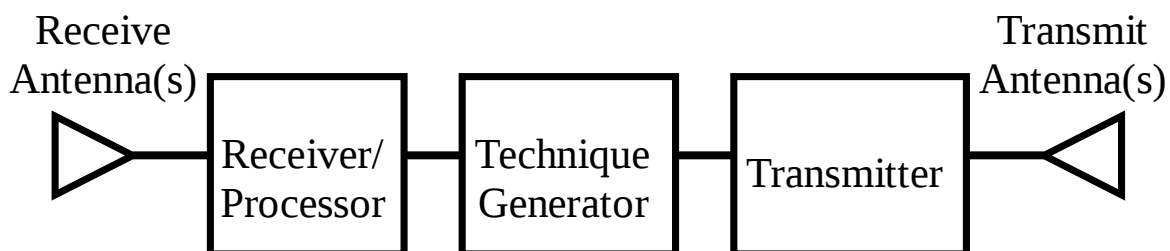
Figure 3-3: Simplified Jammer Block Diagram.
