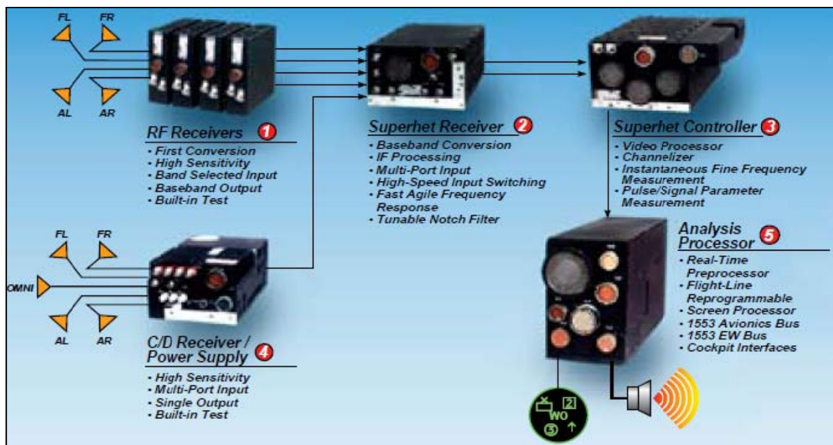
Figure 2-7: RWR Components and Functions – (Courtesy of BAE Systems).
