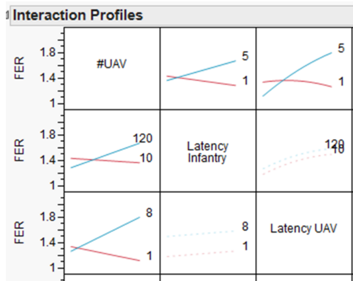
Figure 35. Interaction Plots of UAV Latency vs Number of UAVs
