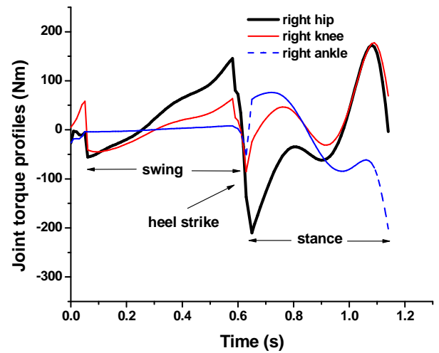
Figure 8. Joint torque profiles of right leg
