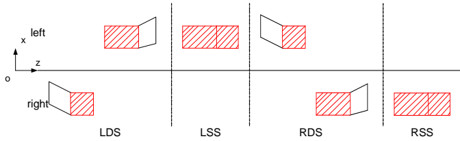
Figure 2. Four basic supporting modes (top view)
