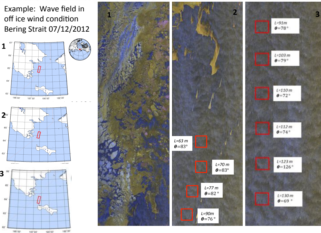
Figure 9: Example of wave and ice measurements from TerraSAR-x satellite observations. Image: T. Lehner and J. Gemmrich (unpublished).
