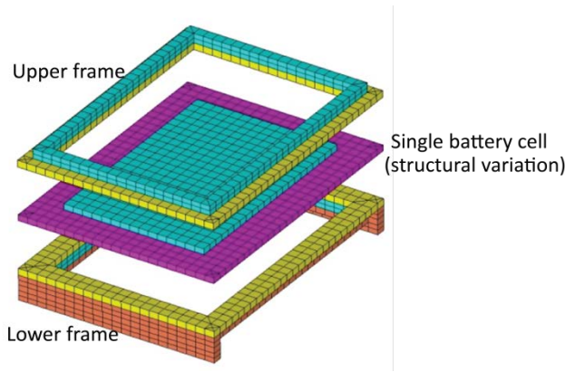
Figure 3. The geometry of a single pouch cell
