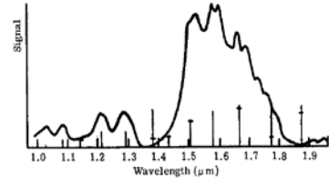
The infrared spectrum
