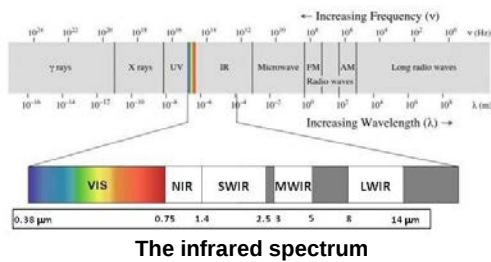
The infrared spectrum
