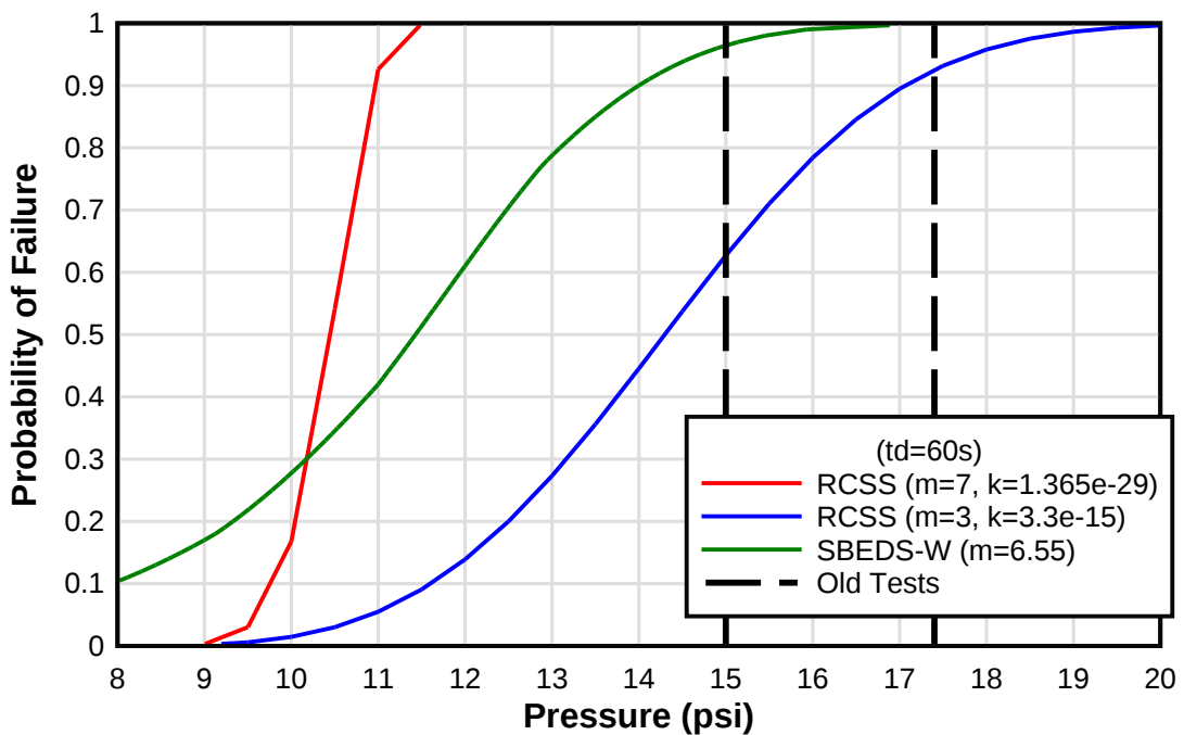
Figure 18. Static Test Validation (39-in x 27-in x 0.190-in Monolithic Hercules® XP)
