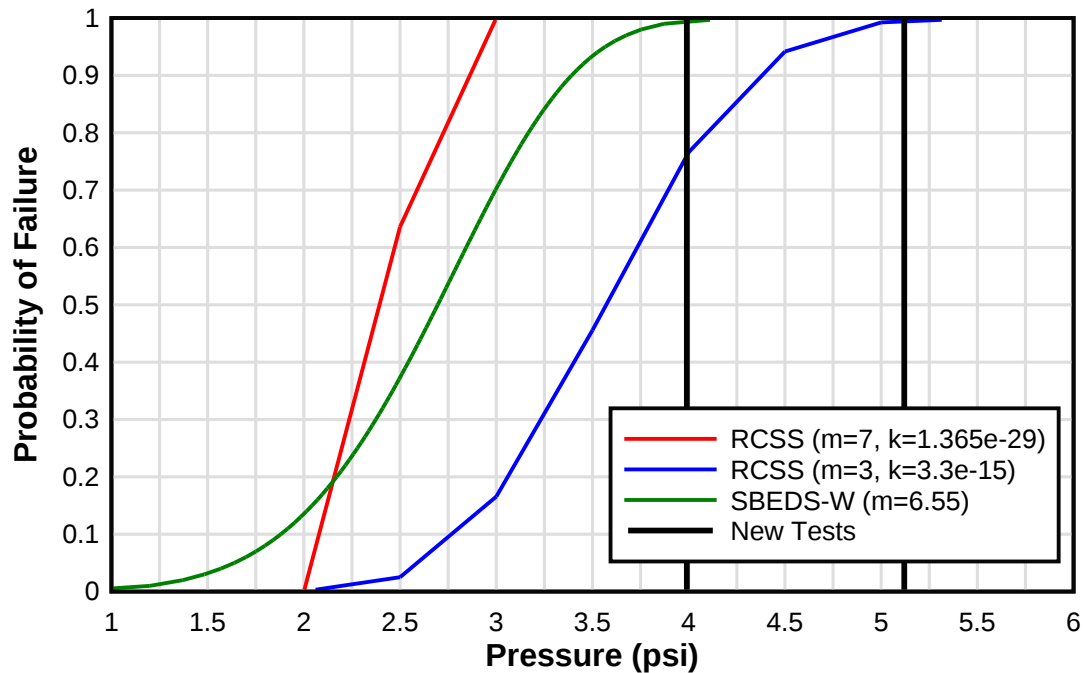
Figure 17. Static Test Validation (60-in x 34-in x 0.115-in Monolithic Hercules® XP)
