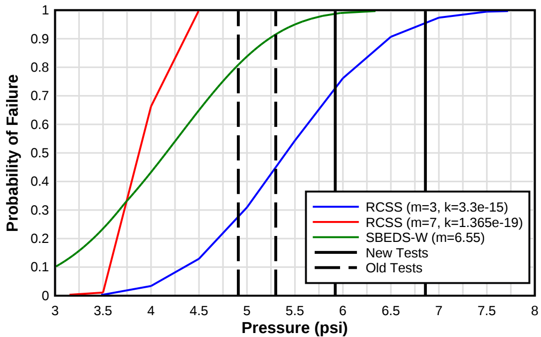
Figure 16. Static Test Validation (60-in × 34-in × 0.155-in Monolithic Herculite® XP)
