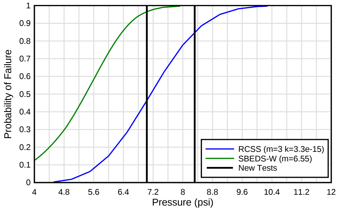
Figure 15. Static Test Validation (60-in × 34-in × 0.180-in Monolithic Herculite® XP)
