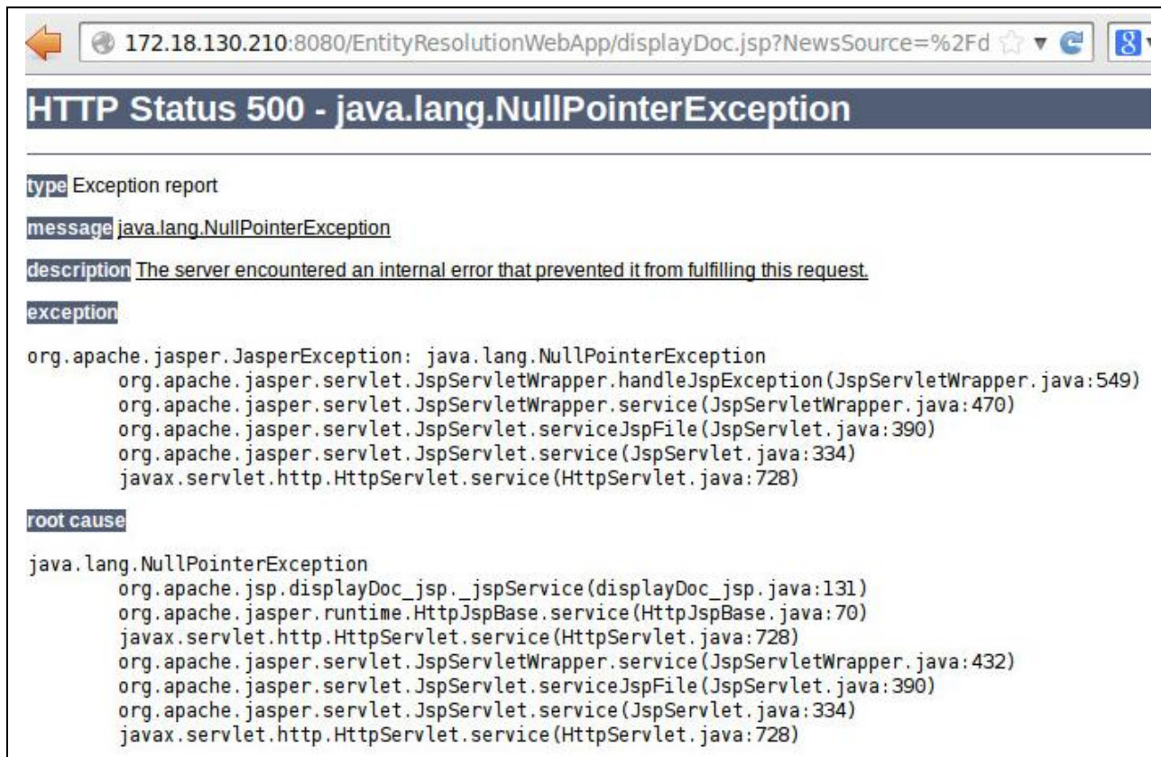
Figure 43. “NullPointerException” error on ERW Web application.
