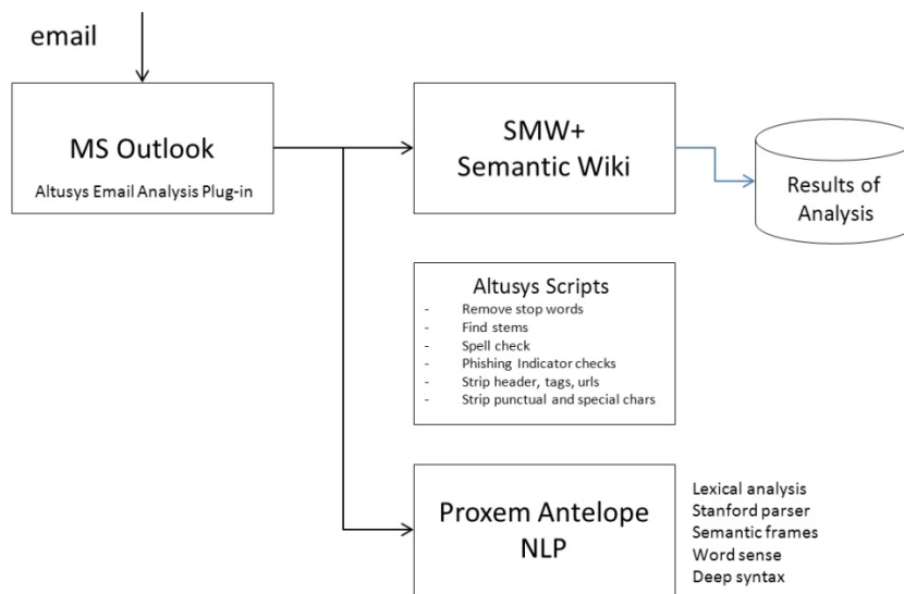
Figure 3 Architecture of prototype system
