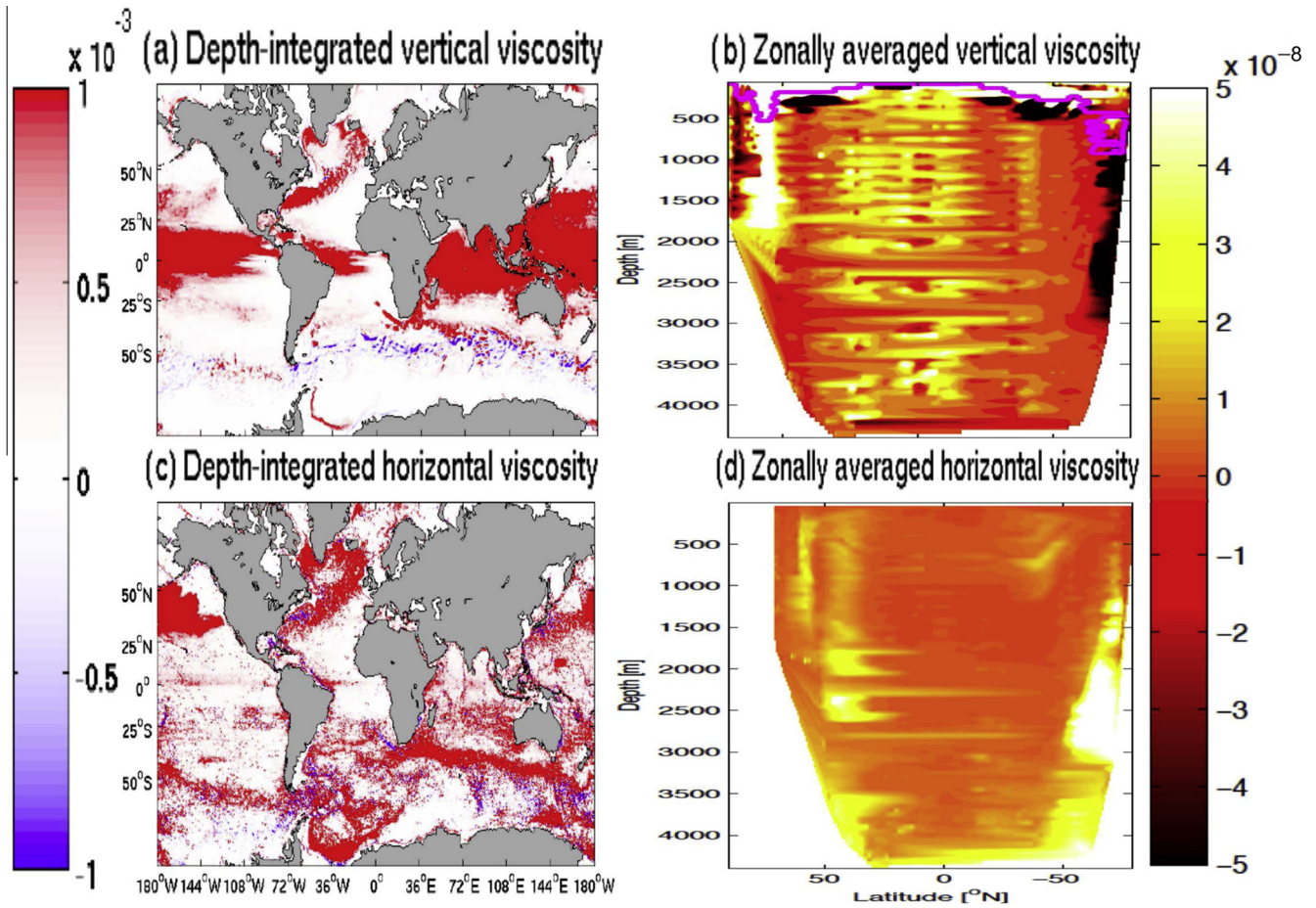
Fig. 6. The (a, b) vertical viscosity and (c, d) “horizontal” viscosity terms in our energy budget, where each viscosity term has units [W m^{-2}] : (a and c) show depth-integrated viscosity terms and (b and d) show zonally-averaged viscosity terms as a function of depth. Shown is an average of inline estimates over the final year of the spin-up phase without wave drag. Listed in Table 2 are the globally integrated power contributions of each term. Shown with magenta contours (panel b) are the deepest mixed layer depths, as determined by KPP, from the final year of the 1/12° HYCOM simulation without wave drag.
