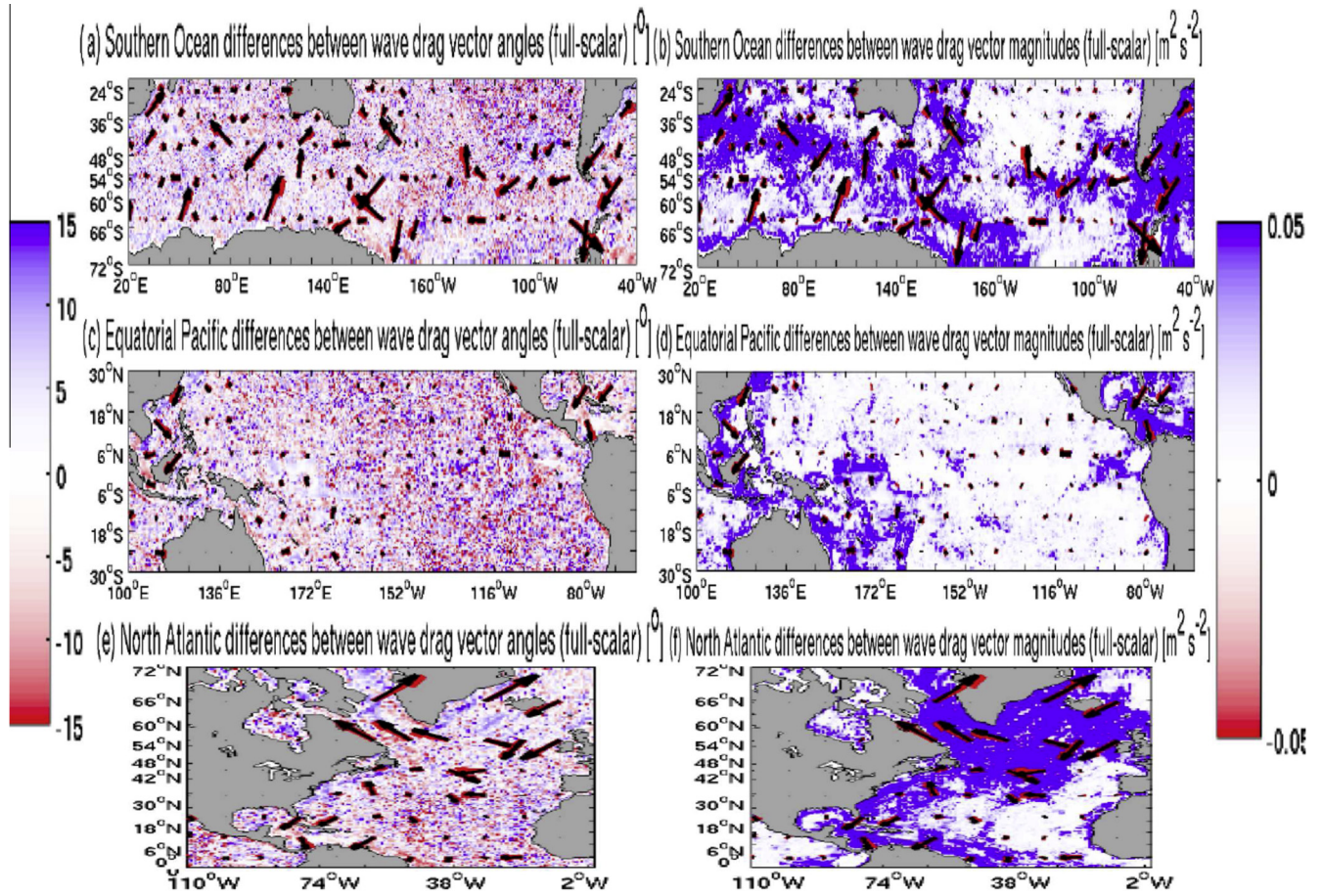
Fig. 4. Offline estimates of the momentum terms associated with wave drag, \bar{\tau}/\rho (black) from (11) and |r_{drag}|\bar{u}_d (red) from (14), in units [m^2 s^{-2}] . Also shown are the (panels a, c, and e) differences between the wave drag vector angles (direction of \bar{\tau}/\rho relative to east minus direction of |r_{drag}|\bar{u}_d relative to east) in units of [\circ] and the (panels b, d, and f) differences between the wave drag vector magnitudes (magnitude of \bar{\tau}/\rho minus magnitude of |r_{drag}|\bar{u}_d ) in units [m^2 s^{-2}] in the Southern Ocean (a, b), equatorial Pacific Ocean (c, d), and North Atlantic Ocean (e, f). Computations shown here were performed with an example five-day average from the last year of the 1/12° HYCOM simulation without wave drag and the vectors are shown separated by ten degree spacings.
