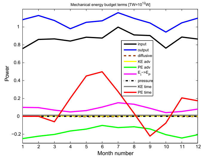
Fig. 14. The seasonal cycle of the estimated power [TW = 10^{12} W] associated with the partial time derivative of kinetic energy ( P_{KE\text{time}} ; “KE time” in legend), the advective flux of kinetic energy ( P_{KE\text{adv}} ; “KE adv”), the partial time derivative of potential energy ( P_{PE\text{time}} ; “PE time”), the advective flux of potential energy ( P_{PE\text{adv}} ; “PE adv”), pressure work ( P_{\text{pressure}} ; “pressure”), buoyancy diffusion ( P_{\text{diffusive}} ; “diffusive”), conversion from internal energy to potential energy ( C_{E_l \rightarrow E_p} ; “ E_l \rightarrow E_p ”), input ( P_{\text{input}} ; “input”), and output ( P_{\text{output}} ; “output”) from the last year of a climatologically forced spin-up of HYCOM with wave drag as a function of climatological month. Here, ‘1’ refers to January, ..., and ‘12’ refers to December.
