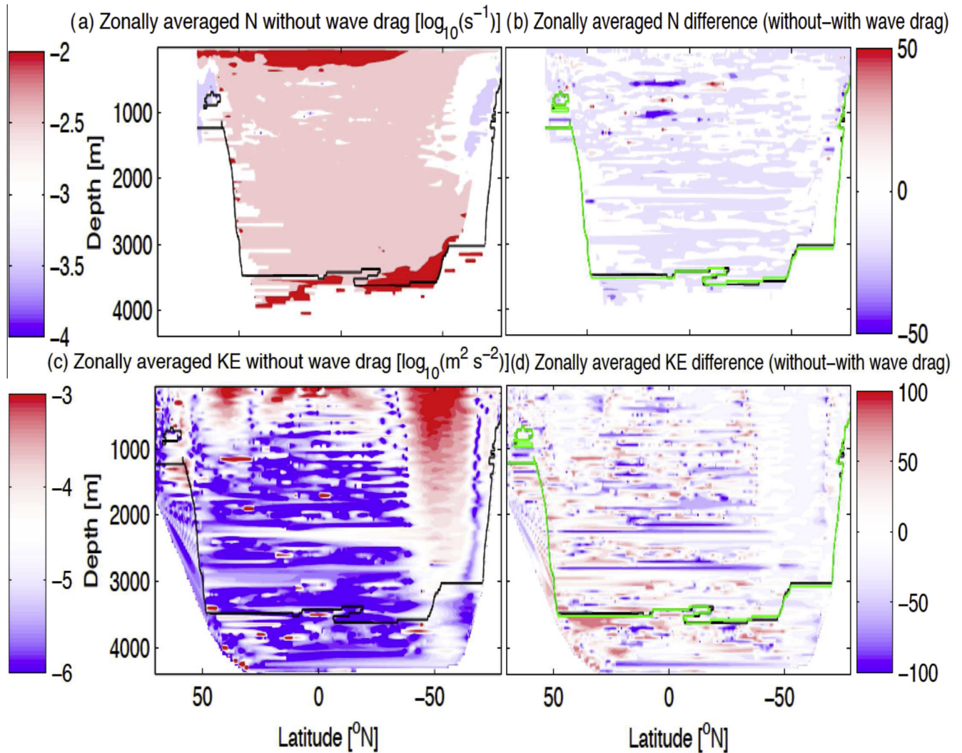
Fig. 12. The (a) \log_{10} of the zonally averaged buoyancy frequency ( N ), which has units [ s^{-1} ], from the 1/12 ^{\circ} HYCOM simulation without wave drag. The (b) percent difference in the zonally averaged N in the 1/12 ^{\circ} HYCOM simulation without wave drag versus in the simulation with wave drag (ratio of their difference to their sum). The (c) \log_{10} of the kinetic energy ( KE ), which has units [ m^2 s^{-2} ], from the 1/12 ^{\circ} HYCOM simulation without wave drag. The (d) percent difference in the zonally averaged KE in the 1/12 ^{\circ} HYCOM simulation without wave drag versus in the simulation with wave drag (ratio of their difference to their sum). Shown with black contours (all panels) are the zonally and temporally averaged depth of the top of the bottom layer in the final year of the 1/12 ^{\circ} HYCOM simulation without wave drag. Shown with green contours (panels b and d) are the zonally and temporally averaged depth of the top of the bottom layer in the final year of the 1/12 ^{\circ} HYCOM simulation with wave drag.
