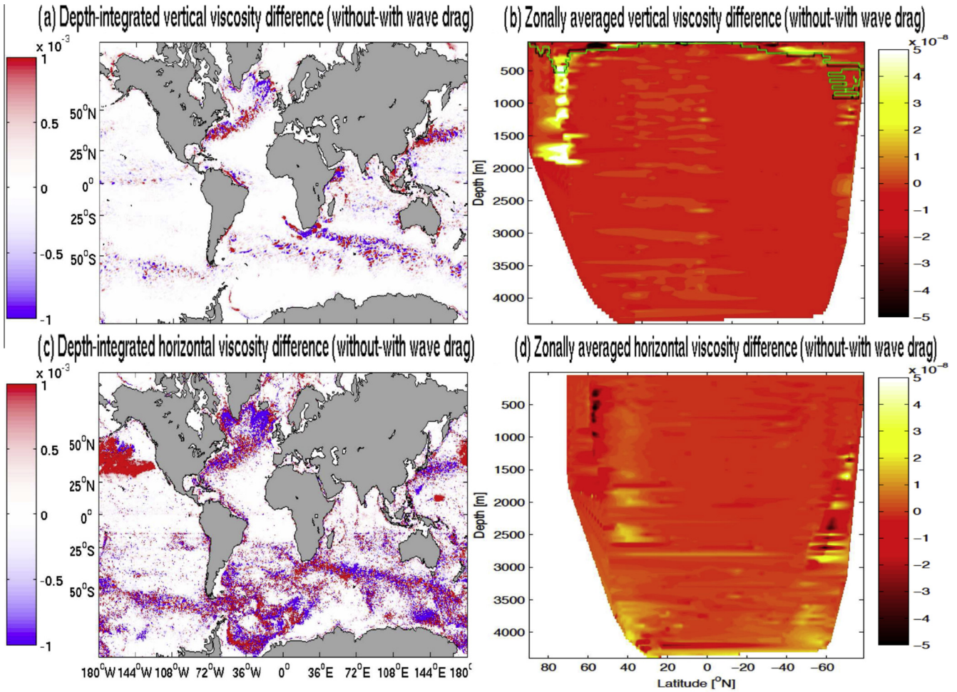
Fig. 8. The average difference in the energy dissipation rates by (a, b) vertical viscosity and (c, d) “horizontal” viscosity terms in our energy budget from the final year of the 1/12^\circ HYCOM simulation without wave drag minus from the final year of the simulation with wave drag, where each panel has units [\text{W m}^{-2}] . Here, (a and c) show depth-integrated viscosity terms and (b and d) show zonally-averaged viscosity terms as a function of depth. Positive values imply a reduction in energy dissipation and negative values imply an increase in energy dissipation upon addition of wave drag to the model. Shown with black contours (panel b) are the deepest mixed layer depths, as determined by KPP, from the final year of the 1/12^\circ HYCOM simulation without wave drag. Shown with green contours (panel b) are the deepest mixed layer depths, as determined by KPP, from the final year of the 1/12^\circ HYCOM simulation with wave drag.
