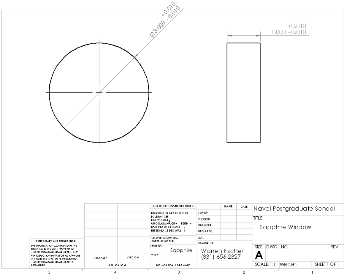
Figure 29. Optical Window Fabrication Drawing
