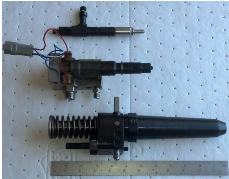
Figure 9. Injectors Used for Testing. From top to bottom: Yanmar injector, Sturman injector, EMD injector.
