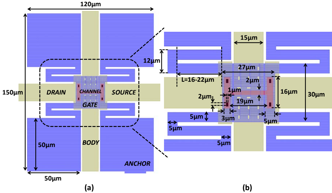
Figure 3.2: 1 st generation 4T relay design. (a) Key dimensions. (b) Zoomed-in view showing channel and dimple regions. Total footprint area is 18000 \mu\text{m}^2 ( 120 \mu\text{m} \times 150 \mu\text{m} ).
