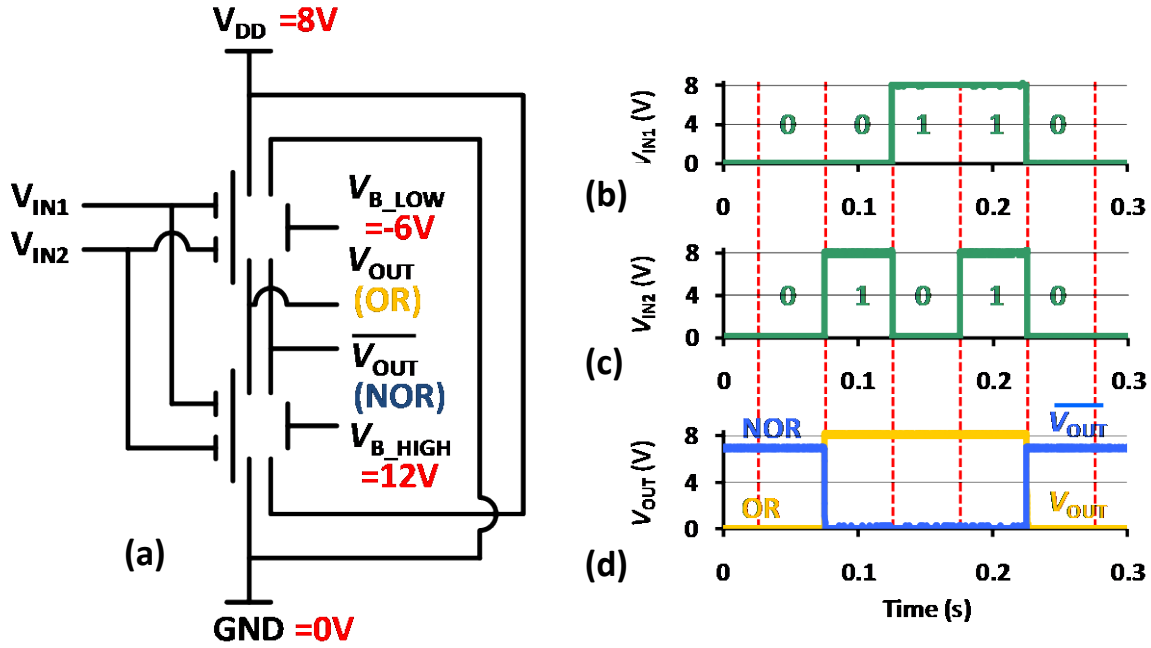
Figure 5.16: Dynamically configurable complementary relay logic circuit utilizing two dual-gate, dual-source/drain relays. (a) Circuit schematic and bias configurations for OR/NOR. V_{DD} = 8 V, V_{B\_HIGH} = 12 V and V_{B\_LOW} = -6 V. (b), (c) Measured input waveform. (d) Measured output waveforms.
