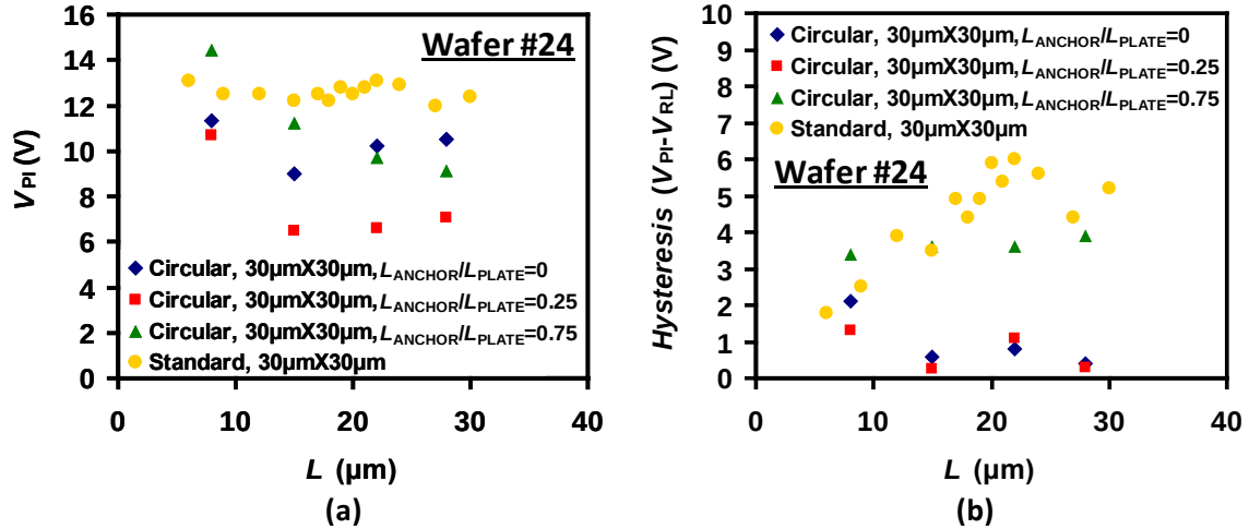
Figure 4.28: Effect of flexure orientation on relay operating voltage. Relay (a) V_{\text{PI}} and (b) hysteresis voltage vs. flexure lengths ( L ) compared for devices with standard and circular flexure orientations. In the circular case, flexures are oriented in a clockwise direction, with the anchor position denoted by L_{\text{ANCHOR}}/L_{\text{PLATE}} ratio (see Figure 4.25(b)). All relays are single-gate, dual-source/drain design with 30 \mu\text{m} ×30 \mu\text{m} plate size from Wafer #24. V_D = 1.5 V, V_S = V_B = 0 V. Tungsten fixed electrode is biased as gate. Process parameters of Wafers #24 are given in Figure 4.8.
