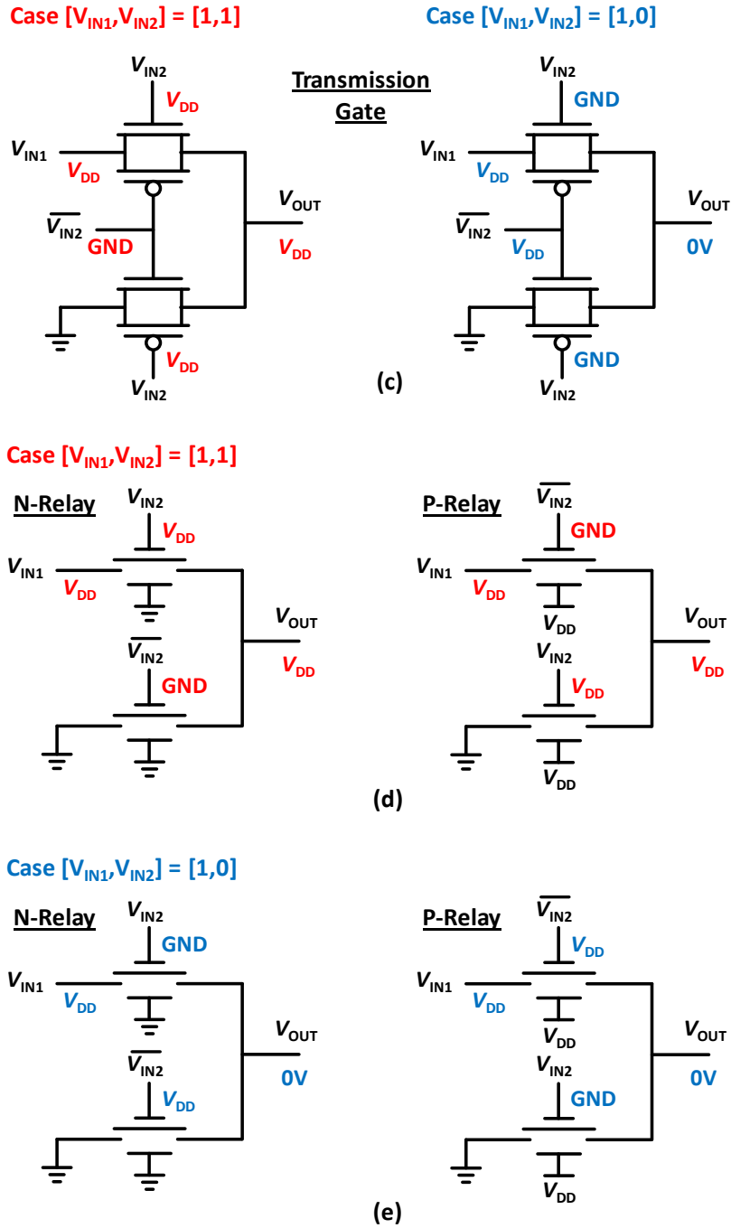
Figure 5.10: Comparison of pass-gate style AND gate implemented with CMOS and relays. Two cases, [V_{IN1}, V_{IN2}] = [1,1] and [1,0] are compared. (a) Pure NMOS and pure PMOS implantation for [1,1] case and (b) [1,0] case. (c) Transmission gate implementation for [1,1] and [1,0] cases. (d) N-relay and P-relay implementation for [1,1] case and (e) [1,0] case.
