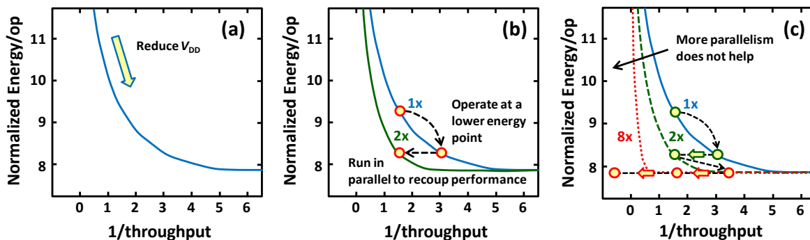
Figure 1.6: Plots of normalized energy per operation vs. 1/throughput demonstrating the benefits of parallelism and its limited effectiveness due to CMOS minimum energy point.
