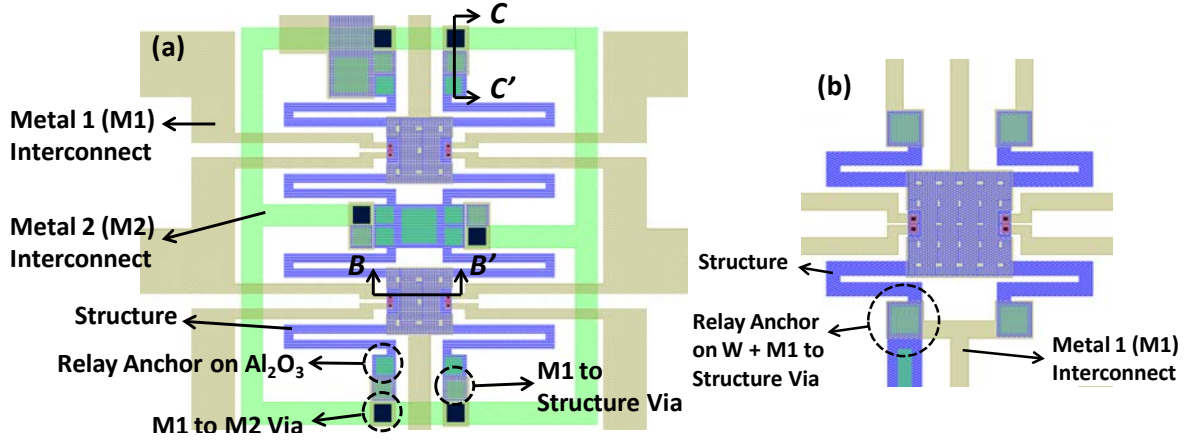
Figure 4.1: Layout view illustrating improved anchor and interconnect design on dual-source/drain devices. (a) An inverter circuit. Relays are anchored on \text{Al}_2\text{O}_3 substrate dielectric. M1 to structure via enables connection from the SiGe structure to the W fixed electrodes. M1 to M2 via provides a connection to an interconnect layer underneath the relay. All flexures are connected through the M2 interconnect, a low resistance path to minimize voltage drops throughout the structure. (b) Device anchored directly on W (M1 interconnect). Combining anchor and via saves area.
