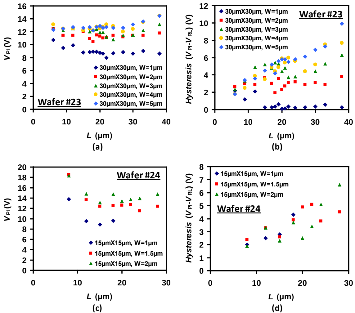
Figure 4.27: Effect of flexure width ( W ) on relay operating voltage. Relay V_{PI} and hysteresis voltage vs. flexure lengths ( L ) compared for various W . (a), (b) 30\mu\text{m} \times 30\mu\text{m} relays from Wafer #23. (c), (d) 15\mu\text{m} \times 15\mu\text{m} relays from Wafer #24. All relays are single-
