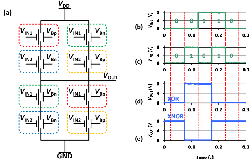
Figure 5.8: A complementary relay XOR/XNOR gate implemented with 4T relays. (a) Circuit schematic for XOR gate. XNOR function can be achieved by simply switching V_{DD} and GND. (b), (c) Measured input waveforms. (d), (e) Measured output waveforms. V_{DD} = 8 V, V_{Bp} = 13 V and V_{Bn} = -5 V. Annotated in different colors are relays that have identical gate and body biases.
