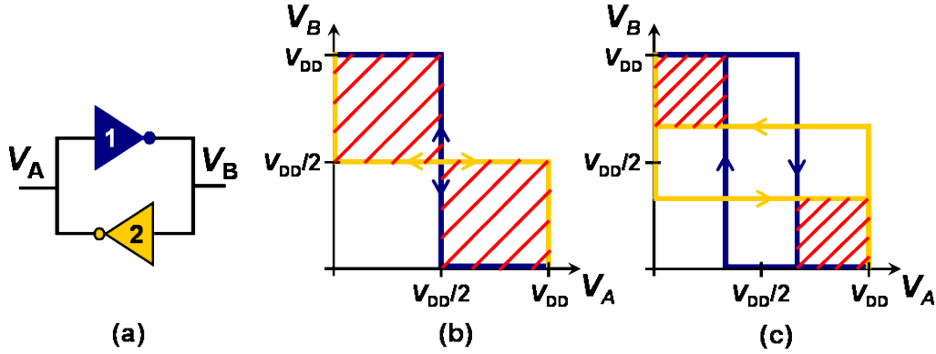
Figure 5.3: Static noise margin (SNM) of digital relay circuit. (a) Basic memory element (latch). (b) Maximum SNM possible is achieved when the voltage transfer characteristic (VTC) has zero hysteresis. (c) Noise margin is reduced with increasing VTC hysteresis.
