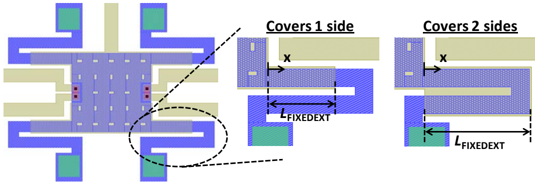
Figure 4.30: Designs with extended fixed (tungsten) electrode areas. The extensions are below the flexures, to provide for extra electrostatic force to actuate the relay. Extension length ( L_{FIXEEXT} ) is measured from the original fixed electrode boundary. Designs that cover 1 side and 2 sides of the flexures are fabricated.
