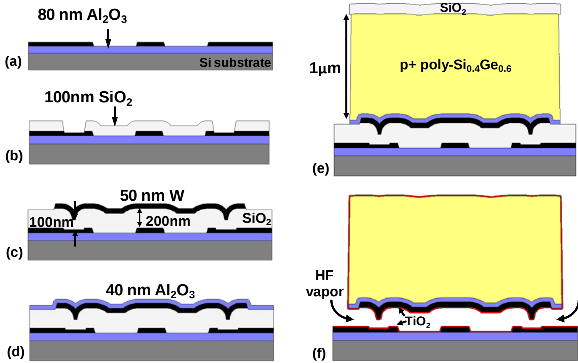
Figure 3.3: Illustration of the 4-mask process used to fabricate the 1 st prototype four terminal relays, shown along cross section A-A' of Figure 3.1. (a) 80 nm \text{Al}_2\text{O}_3 layer deposited and 50 nm W layer deposited and patterned to form source, drain, and body electrodes. (b) 1st sacrificial \text{SiO}_2 layer (100 nm) deposited and source/drain contact regions defined. (c) 2nd sacrificial \text{SiO}_2 layer (100 nm) deposited and 50 nm W layer deposited and patterned to form channel. (d) 40 nm \text{Al}_2\text{O}_3 gate dielectric layer deposited. (e) 1 \mu\text{m} \text{p}^+ poly- \text{Si}_{0.4}\text{Ge}_{0.6} deposited and patterned using LTO hard mask to form gate electrode. (f) Gate-stack released in HF vapor and coated with 3 Å \text{TiO}_2 .
