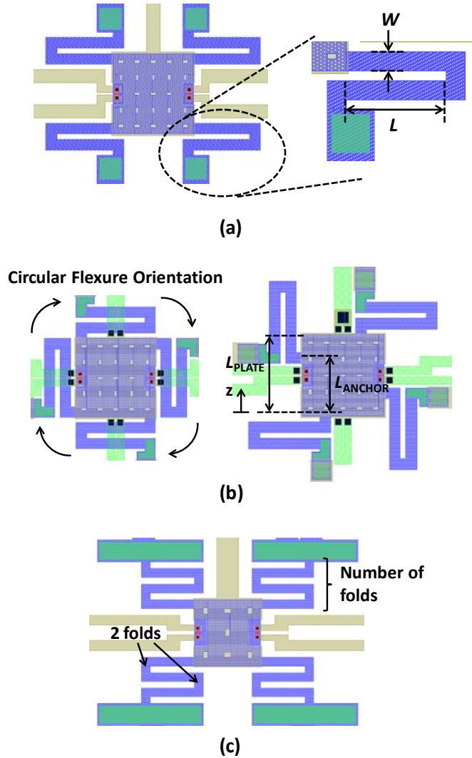
Figure 4.25: Flexure design parameter definition. (a) Definition of flexure width ( W ) and length ( L ). W is the width of the beam which is uniform throughout in all designs. L is defined for one beam section only, not the total beam length. (b) Circular flexure orientation in clockwise direction. In a clockwise orientation, distances ( z ) are measured from one edge of the plate also in a clockwise manner (annotated in the figure). Anchor position is defined by the ratio of the distance of the anchor from the edge of the plate ( L_{\text{ANCHOR}} ) to length of one side of the plate ( L_{\text{PLATE}} ), i.e. L_{\text{ANCHOR}} / L_{\text{PLATE}} . The plates for all designs are square, i.e. L_{\text{PLATE}} is equal for all 4 sides. (c) Definition of number of folds. A relay with 2-fold flexure is shown in (c) vs. standard 1-fold flexure in (a) and (b).
