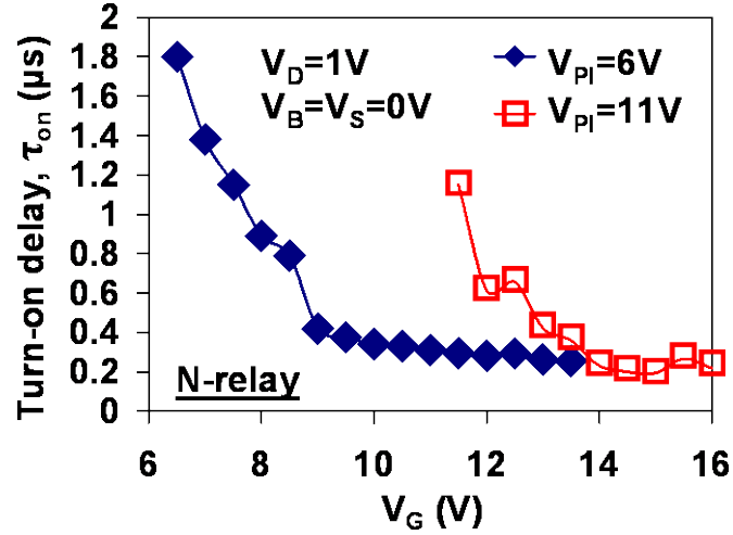
Figure 3.9: Measured turn-on delay ( \tau_{on} ) with increasing applied gate voltage ( V_G ), for two relays with different flexure lengths ( L ). The two relays have V_{PI} = 6V and V_{PI} = 11V . V_D = 1V and V_S = V_B = 0V . Delay decreases with higher V_G , but eventually saturates at \sim 200 ns.
