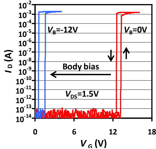
Figure 5.12: Measured I_D - V_G characteristics of a single-gate, dual-source/drain relay with <1 V hysteresis. With body biasing, V_{PI} , can be substantially reduced to <1 V with the relay still able to turn off reliably.
