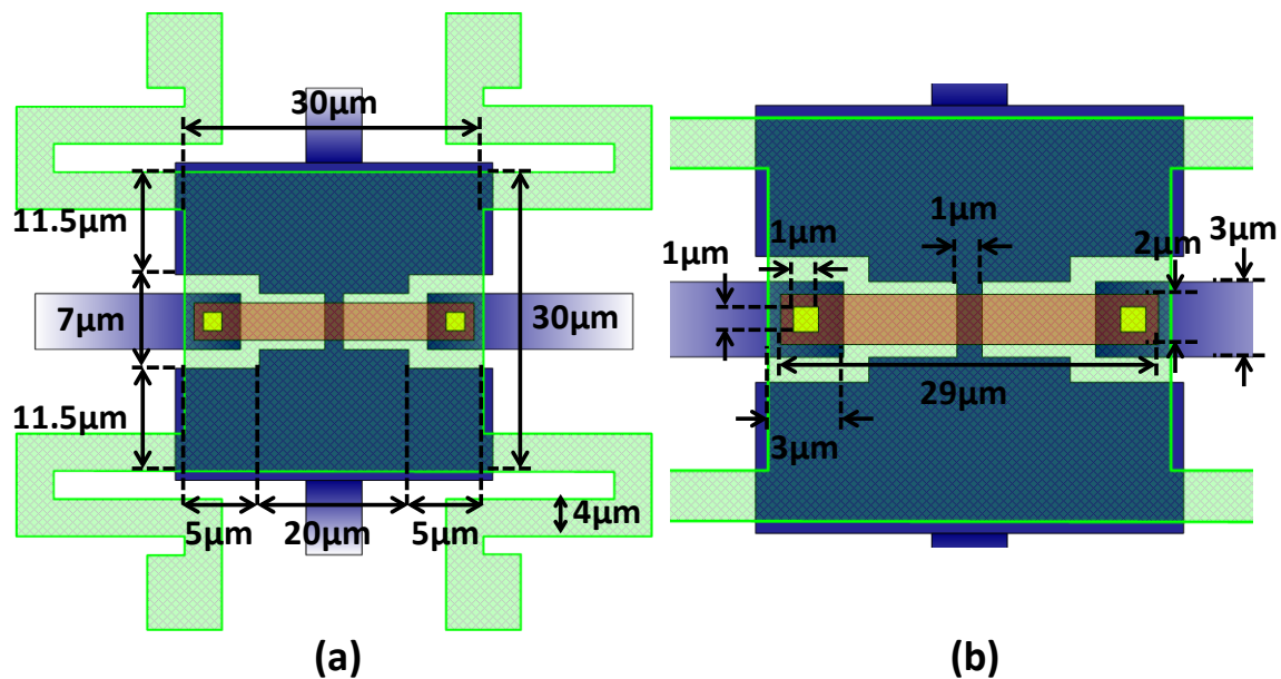
Figure 4.4: 2 nd generation 4T relay design. (a) Key dimensions. (b) Zoomed-in view showing channel and dimple regions. Total footprint size is 68 \mu m \times 78 \mu m.
