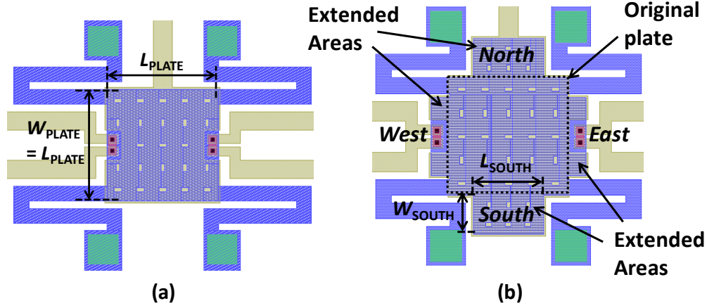
Figure 4.22: Plate design definitions. (a) Plate size for the original design is defined by plate width ( W_{\text{PLATE}} ) and length ( L_{\text{PLATE}} ). Plates are square in all designs presented here, i.e. W_{\text{PLATE}} = L_{\text{PLATE}} . (b) Extended actuation plate designs provides for larger actuation area without any increase in the total device area, because they make use of empty spaces between anchors and flexures. The location of the extension is annotated by “North, South, East, West”, or can be abbreviated by “NSEW”. L_{\text{SOUTH}} \times W_{\text{SOUTH}} denotes the area of the “South” extension. Similar convention applies for the other extensions. Each design is defined by the size of the original plate ( L_{\text{PLATE}} \times W_{\text{PLATE}} ) + total area of the extensions as a percentage of the original plate area.
