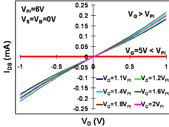
Figure 3.4: Measured I_{\text{DS}}-V_{\text{D}} for V_G < V_{\text{PI}} (off-state) and V_G > V_{\text{PI}} ranging from 1.1V_{\text{PI}} to 2V_{\text{PI}} (on state). Pull-in voltage V_{\text{PI}} = 6\text{V} , V_{\text{S}} = V_{\text{B}} = 0\text{V} .
