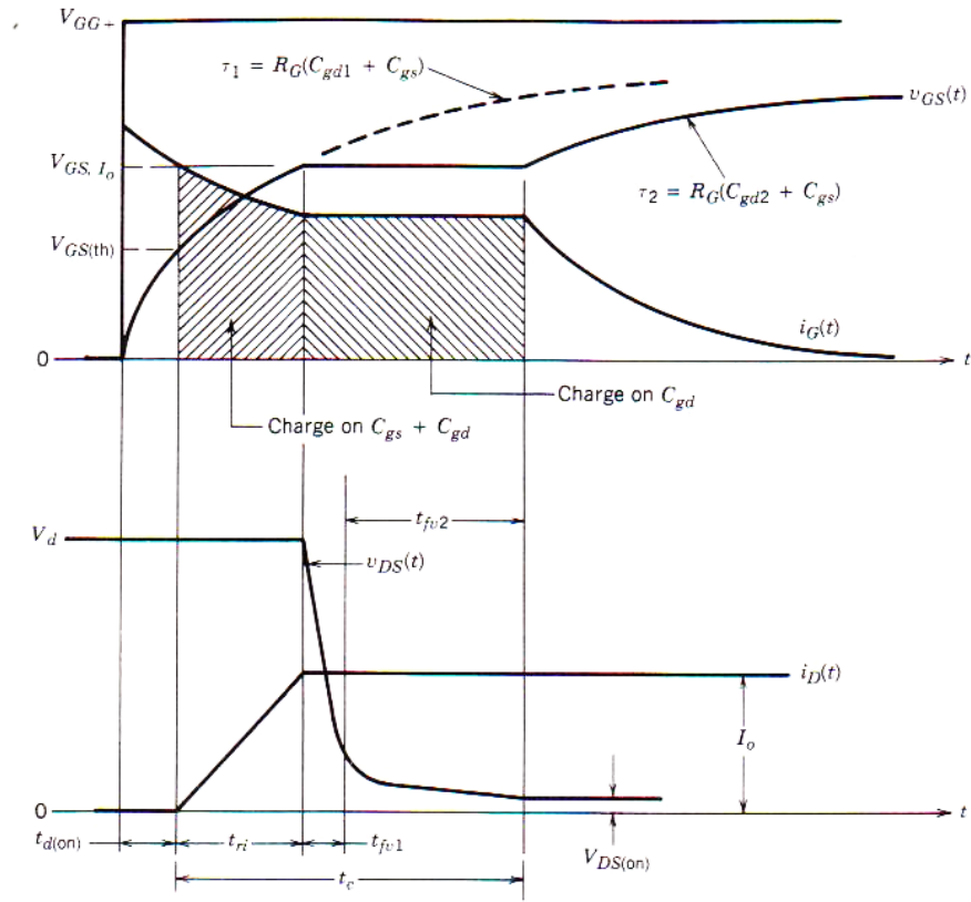
Figure 6. The turn-on voltage and current waveforms of the MOSFET with ideal freewheeling diode. From [8].
