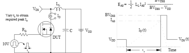
Fig 14. Unclamped Inductive Switching Test Circuit & Waveforms
