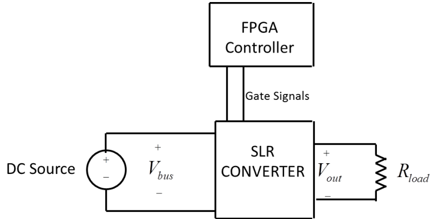
Figure 19. Basic laboratory setup with resistive load used only in Trial 1.
