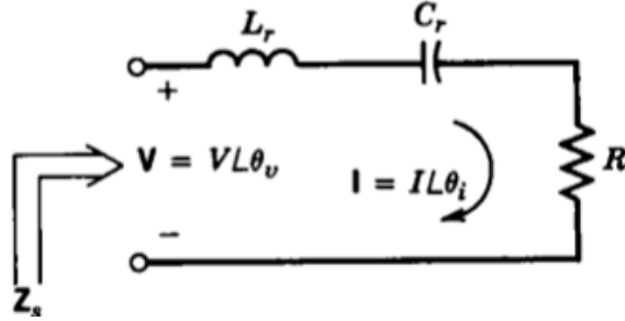
Figure 2. Basic series resonant circuit. From [8].
