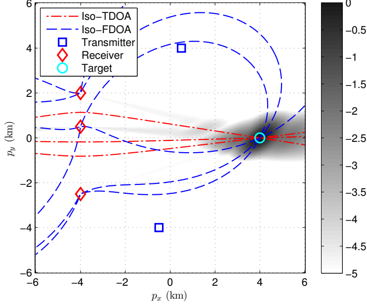
Figure 23. \xi_{ss}(\mathbf{p}, \hat{\mathbf{p}})|_{\hat{\mathbf{p}}=\mathbf{0}} (dB) for \hat{\mathbf{t}} = \mathbf{0} and Six-Element ULA Receivers
