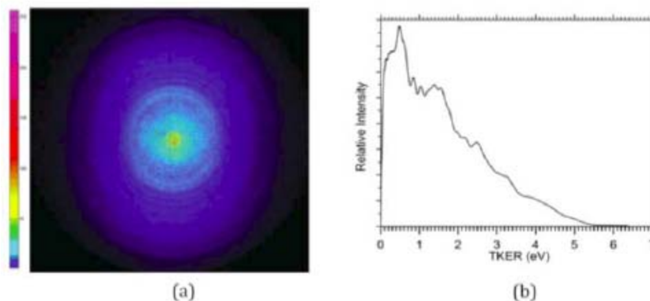
Figure 2. Photodissociation of \text{CO}_2 at 108451.5 \text{ cm}^{-1} . Oxygen atoms in the \text{O}(^1\text{D}_2) state are detected via the autoionization transition 2s^22p^3(^2\text{D}_{3/2}^0)3d\ ^1\text{D}_2 \leftarrow \text{O}(^1\text{D}_2) , (a) The sliced VUV-PI-VMI-image and (b) the P(E_T) derived from the image.
