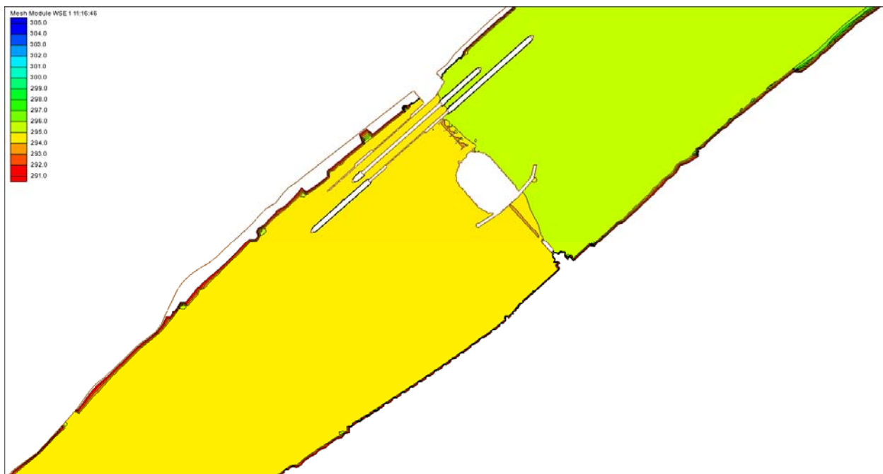
Figure 38. Water surface elevation in feet above the Ohio River Datum for Condition 1.
