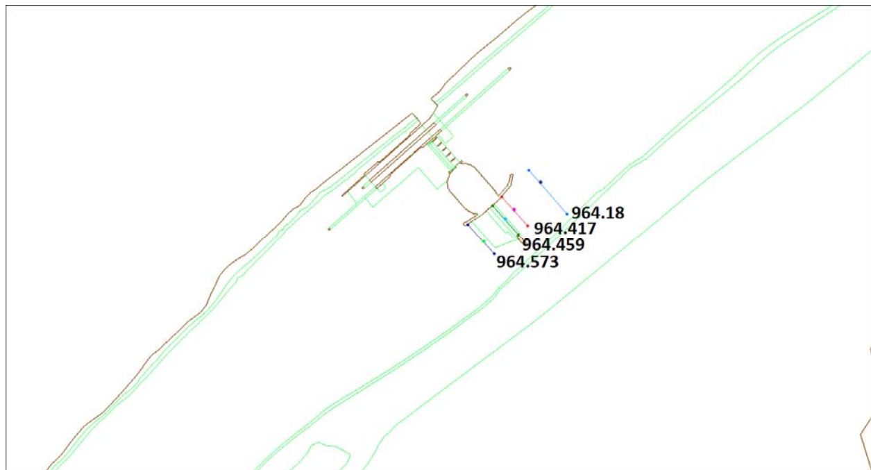
Figure 43. HEC-RAS cross-section locations in the AdH 2012.
