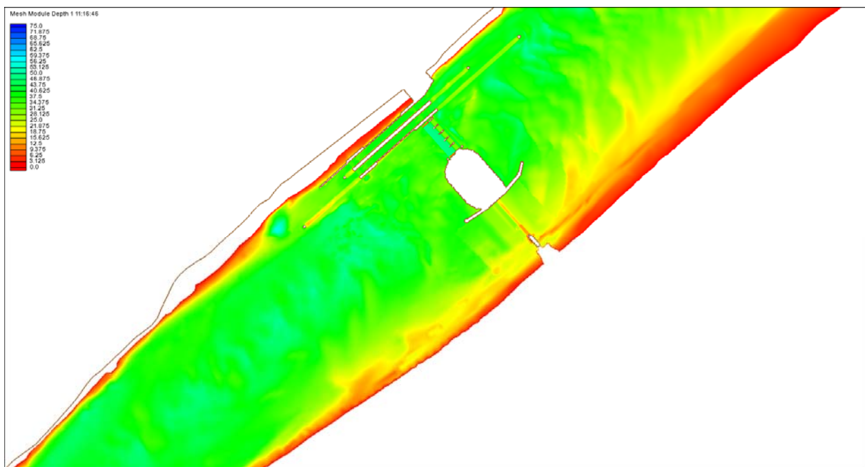
Figure 39. Depth in feet for Condition 1.
