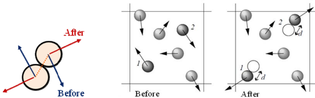
Figure 5: Correlation of relative position and relative velocity in a hard-sphere collision. (left) Displacement of particles in a CBA collision (right)
