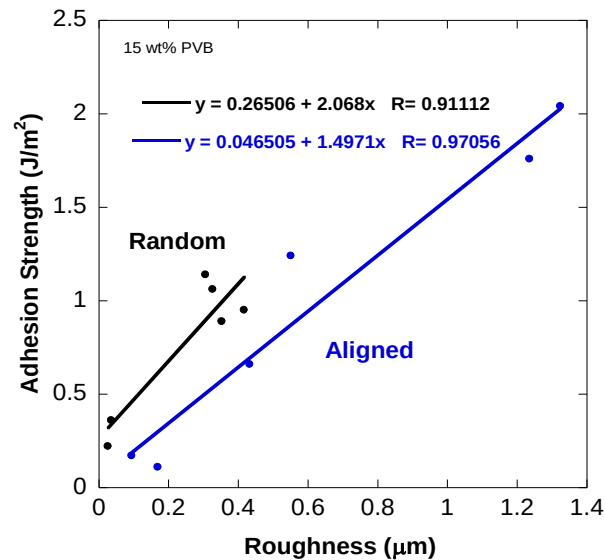
Figure 4.16. Adhesion strength as a function of roughness for randomly and aligned abraded samples
