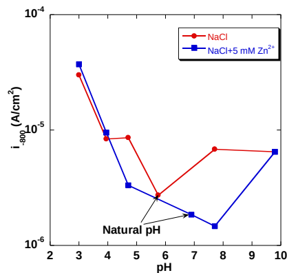
Figure 3.26. Current at -800 V SCE ( i_{-800} ) obtained for two solutions ( 0.1M NaCl with and without additions of 5mM Zn^{2+} inhibitor) at different pH. These data are obtained from polarization studies.
