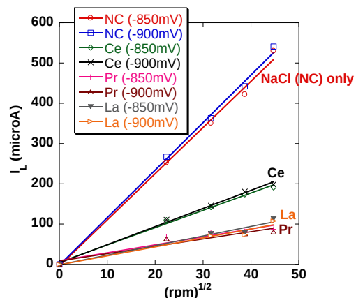
Figure 3.7. Levich representation of the oxygen reduction reaction kinetic data obtained from the polarization curves on Cu RDE in chloride only solutions and chloride solutions containing 100 ppm of the REM cations. (NC stands for 0.1M NaCl solution without any inhibitor additions). The two lines for each cation indicate the data extracted at either - 850 mV SCE or -900 mV SCE .
