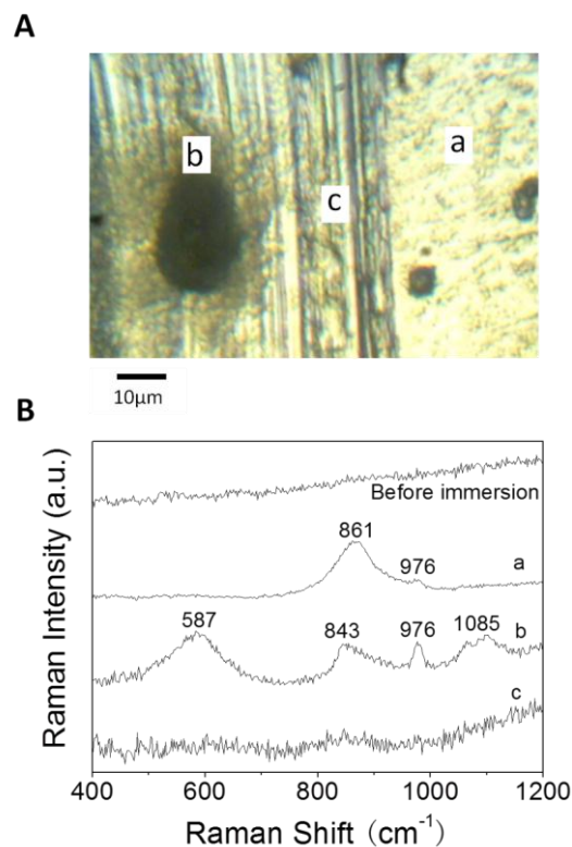
Figure 1.30. (A) Video micrograph of a scratched TCP-coated AA2024 sample after 1-day immersion in 0.5M NaCl + 0.01% (v/v) \text{H}_2\text{O}_2 solution. Afterwards, the scratched sample was rinsed in tap water for 10 s and dried in air at room temperature for 30 min before spectra recording. (B) Raman spectrum of the scratched sample before immersion and spectra after immersion (a) on the coated area, (b) in or near the pitted area in the scratched area and (c) at the terrace site in the scratched area.
