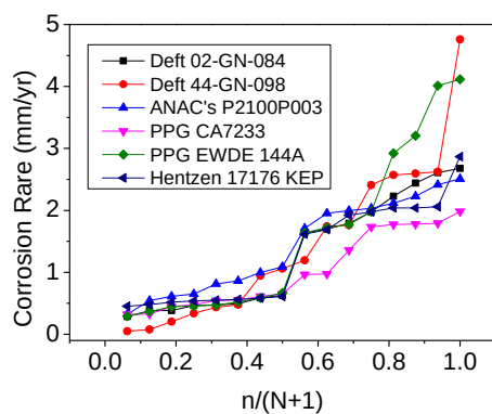
Figure 6.54. Corrosion rate listed by primer in ASTM B117 for 500 h
