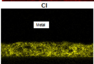
Figure 5.17. Through-film association of chlorine and titanium in Hentzen16708/709 primer following salt spray exposure.
