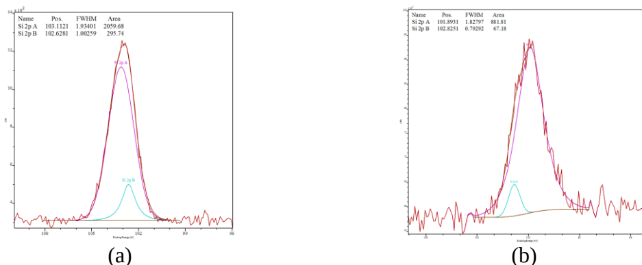
Figure 2.18. The Si 2p spectra for a sample exposed to 0.1 M NaCl solution with and without 25 mM \text{Na}_2\text{SiO}_3 for 24 hours at pH (a) 7.3 and (b) 4.
