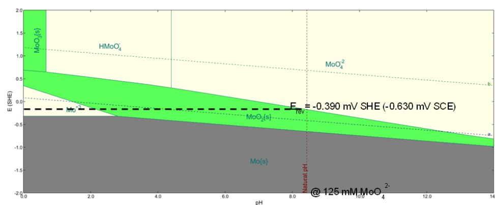
Figure 2.37. Pourbaix diagram of molybdate in aqueous solution at 25°C. Generated using OLI Analyzer.
