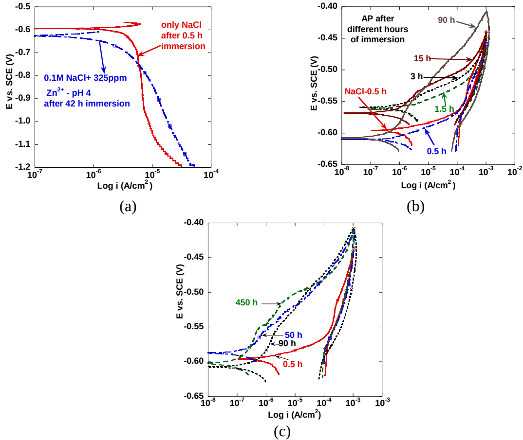
Figure 3.17. (a) Cathodic polarization curve in pH 4 0.1M NaCl solution with 5 mM Zn 2+ after 42hrs immersion (blue curve) against the polarization curve in pH 4 0.1M NaCl solution after 0.5 hours of immersion (red curve) (b) Anodic polarization in pH 4 0.1M NaCl solutions with 5mM Zn 2+ additions after different lengths of immersion time. (c) Anodic polarization of 2024-T3 in chloride-only solutions after different exposure times to test persistence
