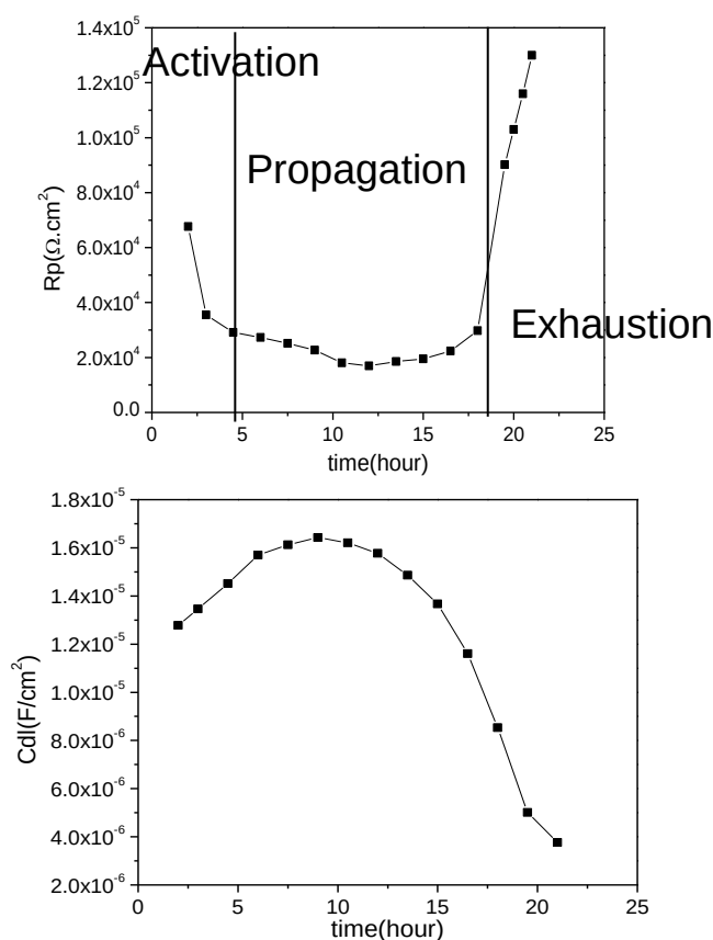
Figure 7.4. (a) Polarization resistance, R_p , and (b) capacitance, C , of an Al thin film metallization with neat epoxy coatings over top. This sample was exposed to 0.3M HCl.
