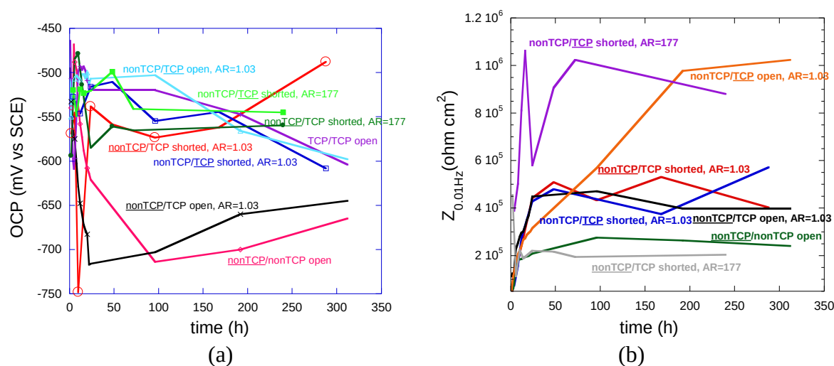
Figure 1.21. Results for TCP coated and non-TCP surfaces in artificial scratch cells containing dilute Harrison's solution under different conditions of shorting and area ratio. "AR" is TCP/non-TCP surface area ratio. "Open" is for non-shorted cell. The surfaces on which the OCP values were measured are underlined, whereas the other surface in the cell is given after the slash. (s) Open circuit potential (b) impedance magnitude at 0.01Hz.
