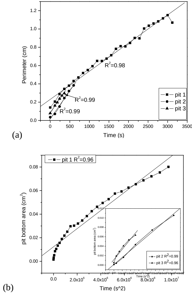
Figure 7.6. Pit perimeter (a) and pit bottom area (b) as a function of time by the image analysis. The closed symbols indicate the original data, the regular lines are the linear fitting results.
