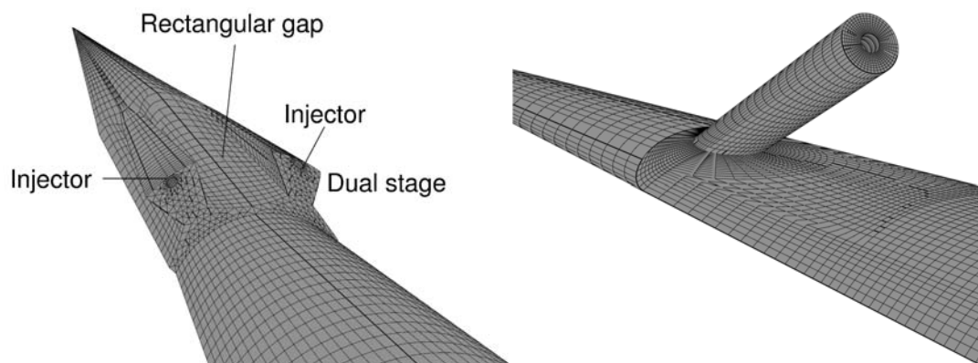
a) Dual stage rectangular gap injector
