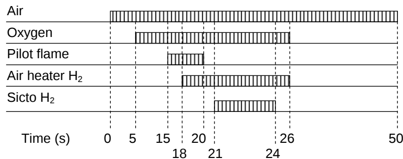
Figure 17: Typical valve sequence of a shock-induced combustion experiment.
