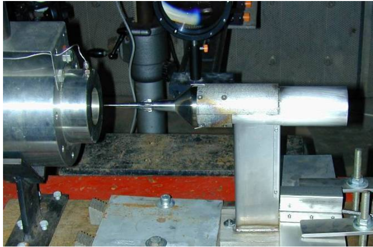
Figure 15: Dual-cone test object mounted behind the TNO free jet test facility.
