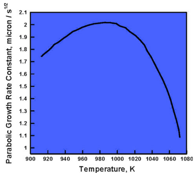
Fig. 6 Temperature dependence of the one-dimensional parabolic growth-rate constant for the austenite \rightarrow allotriomorphic ferrite phase transformation in AISI 1005 (Ref 20)
