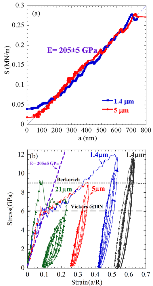
FIG. 4. (Color online) (a) The S vs a curves for the 1.4\ \mu\text{m} and 5\ \mu\text{m} tips. (b) Typical NI stress-strain curves obtained after a given location was indented to the highest loads ( 550\ \text{mN} for 21\ \mu\text{m} , 100\ \text{mN} for 5\ \mu\text{m} , and 20\ \text{mN} for 1.4\ \mu\text{m} tips) for two cycles, unloaded and progressively loaded to higher stresses to obtain the nested loops (three left curves). Plot shown on extreme right shows the reproducible NI stress-strain loops for 1.4\ \mu\text{m} indenter; it was shifted to the right from its original position for clarity. Dashed horizontal and inclined lines represent the Vickers microhardness, Berkovich hardness, and elastic moduli obtained from the S vs a curves, respectively. Pop-ins were only observed when the 21\ \mu\text{m} tip indenter was used.
