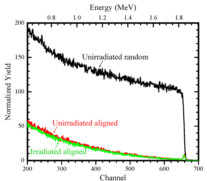
FIG. 8. (Color online) RBS spectra from unirradiated random, unirradiated aligned, and irradiated aligned. The \chi_{\text{min}} = 1.5\% (ratio of aligned to random yield just below the surface peak) indicated very good quality of the unirradiated sample. The aligned spectrum did not change after irradiation because the concentration of defects in the near surface region is quite small.
