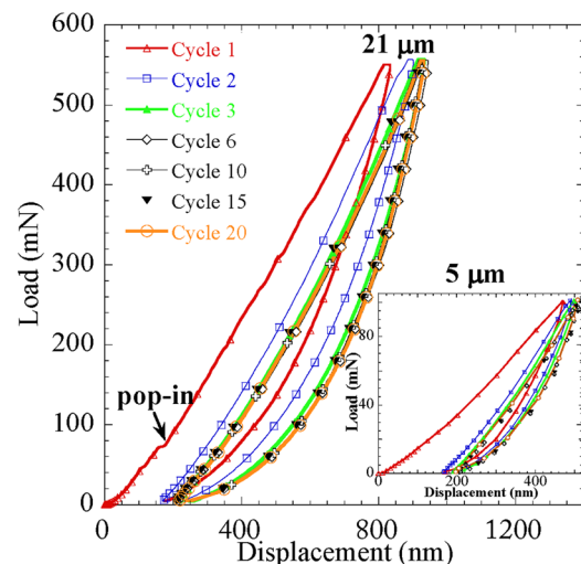
FIG. 2. (Color online) Typical NI load-displacement curves when an unirradiated C-plane LiTaO 3 single crystal is loaded 20 times to 550 mN with the 21 \mu\text{m} radius indenter. Note presence of small pop-ins. Bottom right inset shows the same plot for the 5 \mu\text{m} radius tip loaded twenty times to 100 mN. In both cases, for clarity's sake, only a few cycles are plotted.
