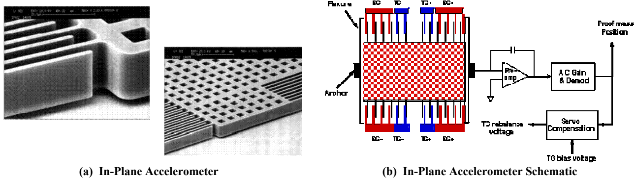
Figure 6. MEMS Lateral Accelerometer
