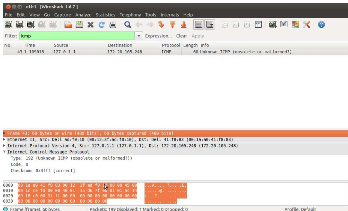
Figure 17. Wireshark capture of ICMP type 192 packet
