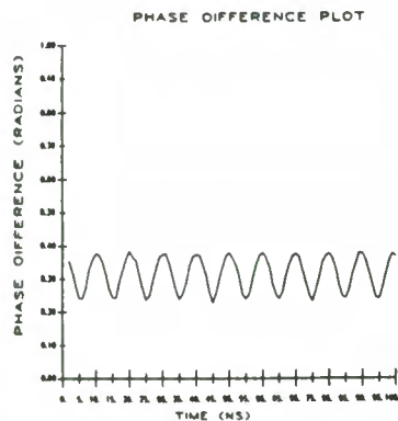
Fig 5. Two simultaneous signals: 50 and 150 MHz
