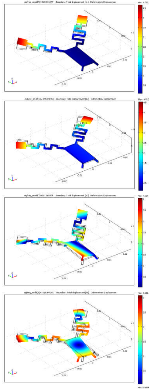
Figure 7. Eigenmodes for the complete jitterbot at (top to bottom) 320, 424, 861 and 1016 Hz.
