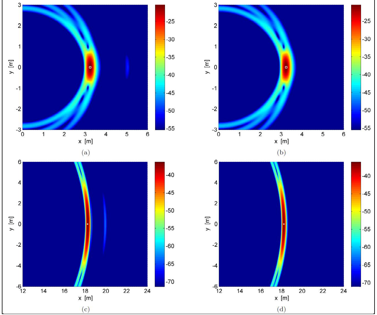
Figure 2. Comparison of FDTD- and MoM-simulated imaging results for an on-surface, perfectly-conducting cube at two ranges: (a) FDTD: range=3.24 m; (b) MoM: range=3.24 m; (c) FDTD: range=18.24 m; and (d) MoM: range=18.24 m. Ground properties: \epsilon_r=6 , \sigma_d=10 mS/m. Frequency span: 0.1–1.4 GHz.
