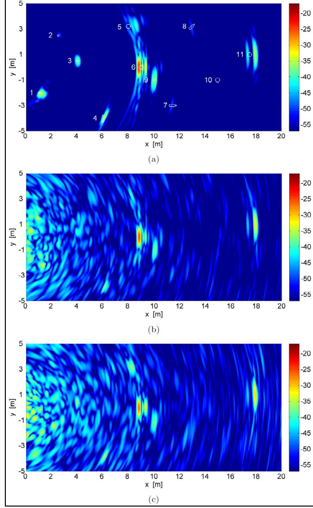
Figure 4. Simulated vertical-vertical (vv)-polarized images for 20 m×10 m scene: (a) Ground with flat surface; (b) Ground with randomly rough surface, h_{rms}=1.2 cm, l_c=14.93 cm; (c) Ground with randomly rough surface, h_{rms}=1.6 cm, l_c=14.93 cm. Ground electrical properties: \epsilon_r=6 , \sigma_d=10 mS/m. Frequency span: 0.3–1.5 GHz.
