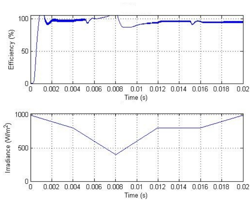
Figure 5.31: InC Run 8. Converter efficiency (top) and irradiance (bottom) versus time.
