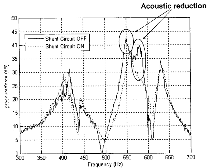
Figure 21. Acoustic response of prototype #3 – Baseline, multiple actuators.
