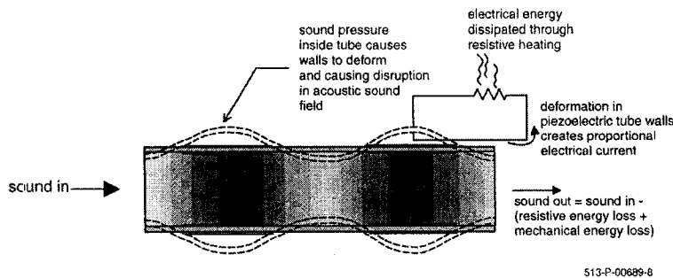
Figure 2: The Foster-Miller Smart Exhaust System (SES) Concept.
