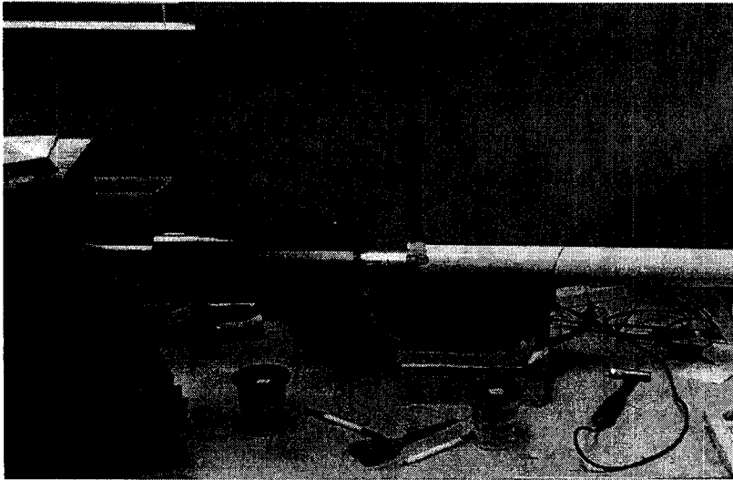
Figure 19. Vibration and acoustic test setup, showing the acoustic source in an acoustically isolated box (at left of picture).
