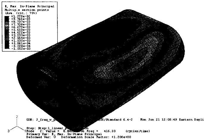
Figure 5. Elastic strain of first noise generating mode (1:1).
