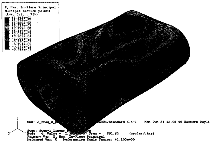
Figure 6. Elastic strain of second noise generating mode (2:1).
