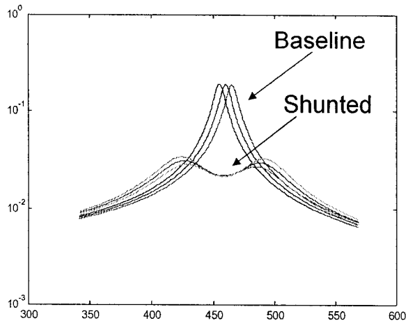
Figure 15. Matlab prediction of the shunted RL-circuit.
