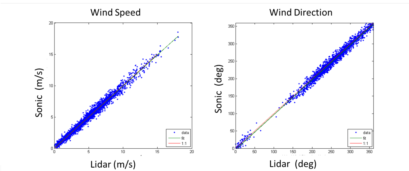
Figure 5 A comparison of wind speed (left) and direction (right) as measured by the bow mounted NOAA Sonic and HRDL wind profile results at a similar height. The sonic data were averaged to the same time resolution as the lida profiles: 20 minutes.
