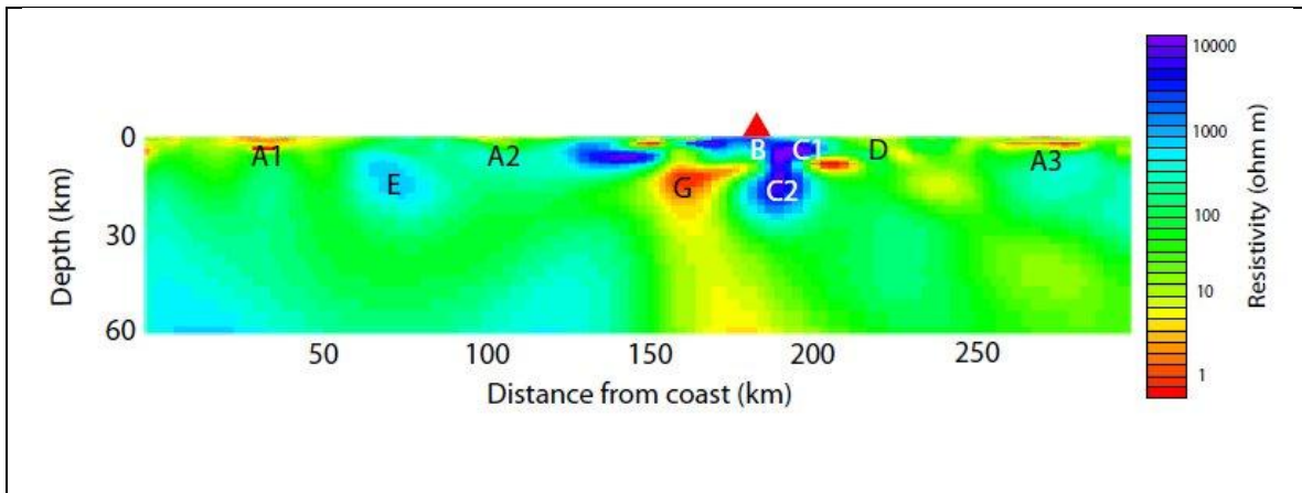
Figure 8: The upper 60 km of the conductivity structure for the CAFE line. The red triangle marks the location of Mt. Rainier just to the south of the profile. A1-A3 mark conductors associated with sedimentary basins. B, C1, and C2 are resistive features associated with Mt. Rainier and the Western Cascades. D is a conductive feature beneath the High Cascades. The resistor E is associated with the crustal forearc, and we interpret the strong conductor G as a magma chamber feeding Mt. Rainier.
