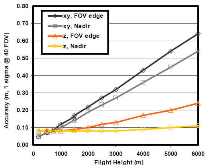
Figure 6: Leica ALS60 Horizontal and Vertical Error Curve
