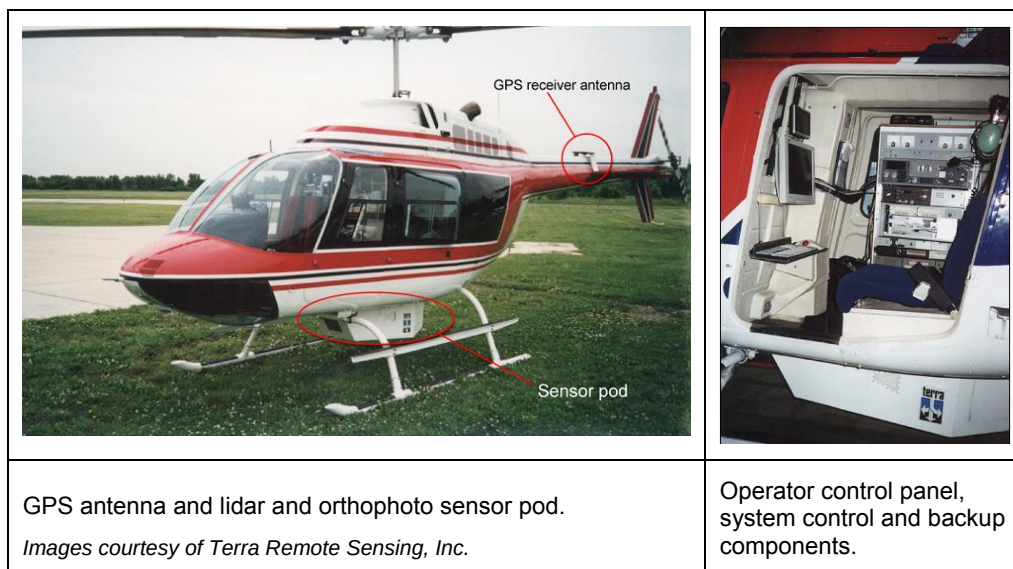
Figure 2: Helicopter-Mounted Lidar and Orthophoto System
