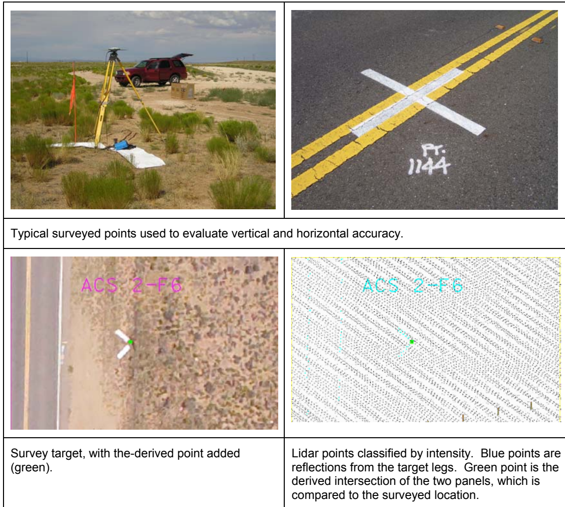
Figure 1: Surveyed Control Points Used to Assess Vertical Error
