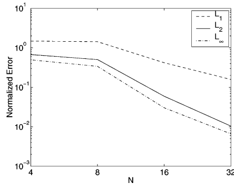
Fig. 4. Case 1B. The normalized \phi error norms for SESL as a function of N after 12 days using n_H = 1 .
