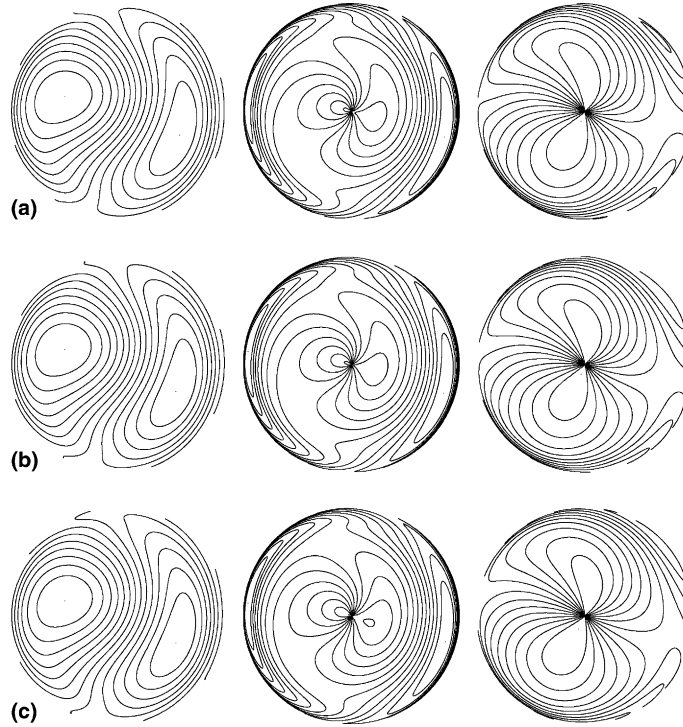
Fig. 14. Case 4. Contours of \phi (left), u_s (center), and v_s (right) for: (a) SEM-LF, (b) SESI, and (c) SESL after 10 days using n_H = 4 and N = 16 .
