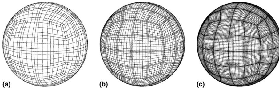
Fig. 1. A hexahedral grid for n_H = 4 and (a) N = 4 , (b) N = 8 , and (c) N = 16 .
