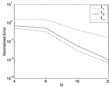
Fig. 2. Case 1A. The normalized \varphi error norms for SESL as a function of N after 12 days using n_H = 1 .
