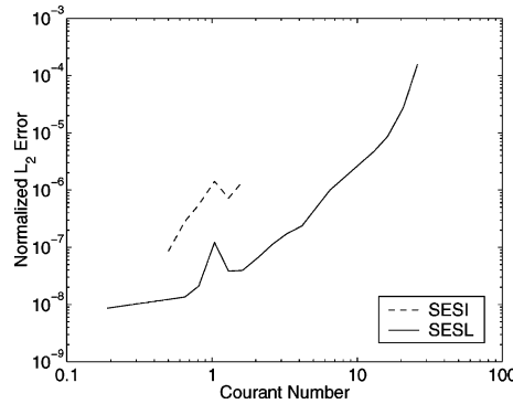
Fig. 13. Case 3. The normalized \phi L_2 error norm for SESI (dashed) and SESL (solid) as a function of Courant number after five days using n_H = 4 and N = 16 .
