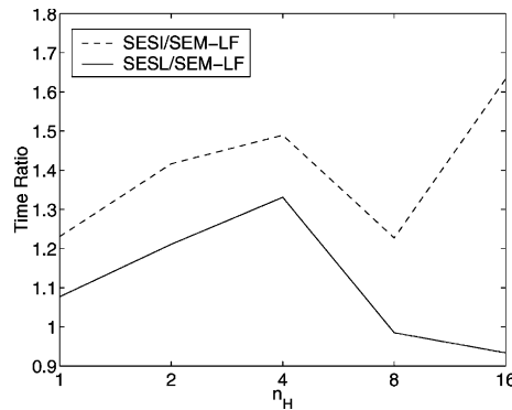
Fig. 18. The ratio of computational cost for SESI/SEM-LF (dashed) and SESL/SEM-LF (solid) for various n_H for Case 5 using N = 8 . The ratios reflect the amount of computer time required to complete a 24 h time-integration.
