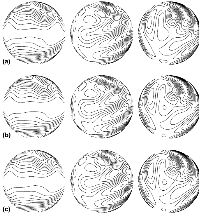
Fig. 15. Case 5. Contours of \varphi (left), u_s (center), and v_s (right) for: (a) SEM-LF, (b) SESI and (c) SESL after 15 days using n_H = 4 and N = 16 .
