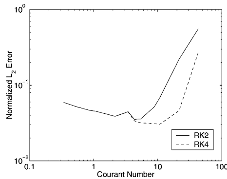
Fig. 5. Case 1B. The normalized \phi L_2 error norm for SESL using RK2 (solid) and RK4 (dashed) for the trajectory computation as a function of Courant number after 12 days using n_H = 1 and N = 16 .
