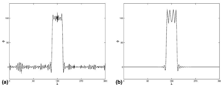
Fig. 8. Case 1C. The mass \varphi along the Equator after 12 days using n_H = 4 and N = 16 for: (a) SESI and (b) SESI with filtering.
