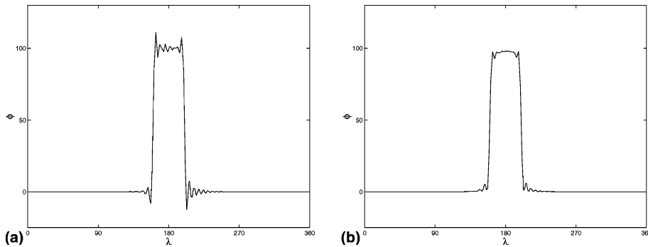
Fig. 9. Case 1C. The mass \varphi along the Equator after 12 days using n_H = 4 and N = 16 for: (a) SESL and (b) SESL with FCT.
