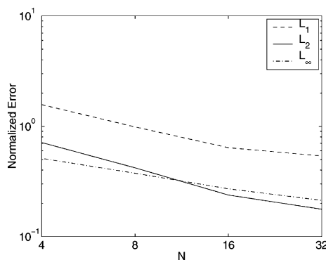
Fig. 6. Case 1C. The normalized \varphi error norms for SESL as a function of N after 12 days using n_H = 1 .
