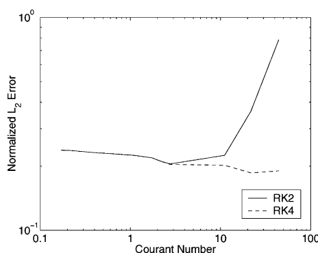
Fig. 7. Case 1C. The normalized \varphi L_2 error norm for SESL using RK2 (solid) and RK4 (dashed) for the trajectory computation as a function of Courant number after 12 days using n_H = 1 and N = 16 .
