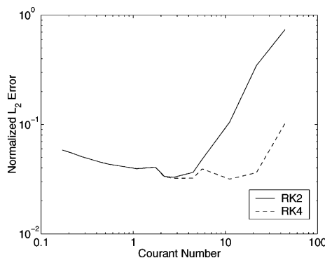
Fig. 3. Case 1A. The normalized \varphi L_2 error norm for SESL using RK2 (solid) and RK4 (dashed) for the trajectory computation as a function of Courant number after 12 days using n_H = 1 and N = 16 .
