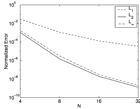
Fig. 10. Case 2. The normalized \phi error norms for SESL as a function of N after five days using n_H = 1 .
