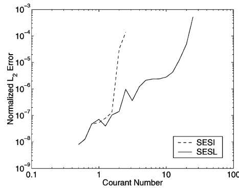
Fig. 11. Case 2. The normalized \phi L_2 error norm for SESI (dashed) and SESL (solid) as a function of Courant number after five days using n_H = 4 and N = 16 .
