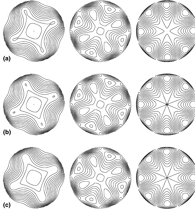
Fig. 16. Case 6. Contours of \varphi (left), u_s (center), and v_s (right) for: (a) SEM-LF, (b) SESI and (c) SESL after 14 days using n_H = 4 and N = 16 .
