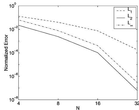
Fig. 12. Case 3. The normalized \phi error norms for SESL as a function of N after five days using n_H = 1 .
