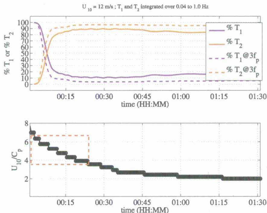
FIG. 4. (top) Contribution of T_1 vs T_2 to the total dissipation for the UL1M4 U_{10} = 12 \text{ m s}^{-1} simulation. The integrated T_1 and T_2 values (solid lines) and the values at 3f_p (dashed lines). (bottom) Inverse wave age for the same simulation. Wave age and time period corresponding to the Manasseh et al. (2006) study are indicated (dashed-line box).
