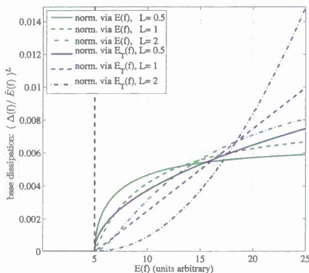
FIG. 2. Qualitative demonstration of expected impact of the choice of normalization variable and choice of power coefficient L . The vertical axis shows a dissipation quantity that has been normalized by the total area under each curve in the region plotted to aid viewing and roughly approximate the effect of calibration. Here, only one frequency is shown, and the E_T at this frequency is 5 (units are unimportant here), so dissipation is zero for E < 5 .
