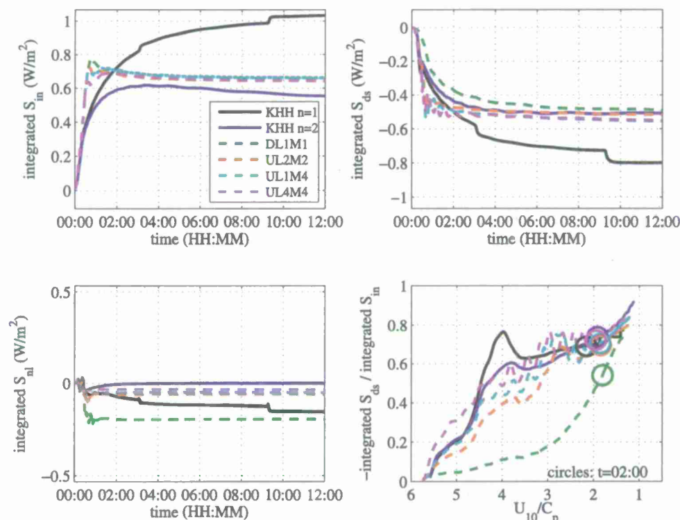
FIG. 7. Frequency-integrated source terms. Models shown are the same as those shown in Fig. 3. (bottom right) The ratio between dissipation and input vs inverse wave age is shown, with circles indicating the points 2 h into each simulation. The frequency range for the integration is 0.042–1.0 Hz.
