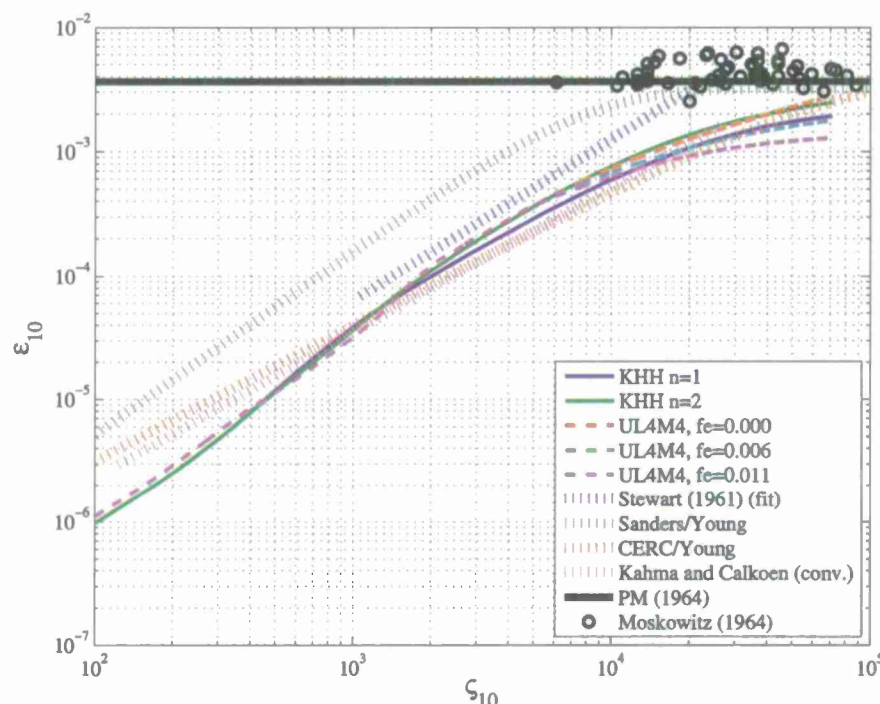
FIG. 8. Verification of duration-limited growth rate (energy vs time). Both quantities are nondimensionalized using U_{10} . Two models based on KHH, three new observation-consistent models (UL4M4), four empirical growth curves (described in the text), the PM limit and PM values are shown.
